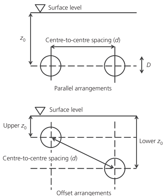
Figure 1. Illustration of the various twin-tunnel arrangements tested
