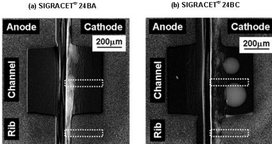
Figure 3 Cross-sectional images of water accumulation under channel and rib area at current density of 0.8 \text{ A cm}^{-2} for (a) SIGRACET® 24BA; and (b) SIGRACET® 24BC h (Reproduced from [131] with permission)
