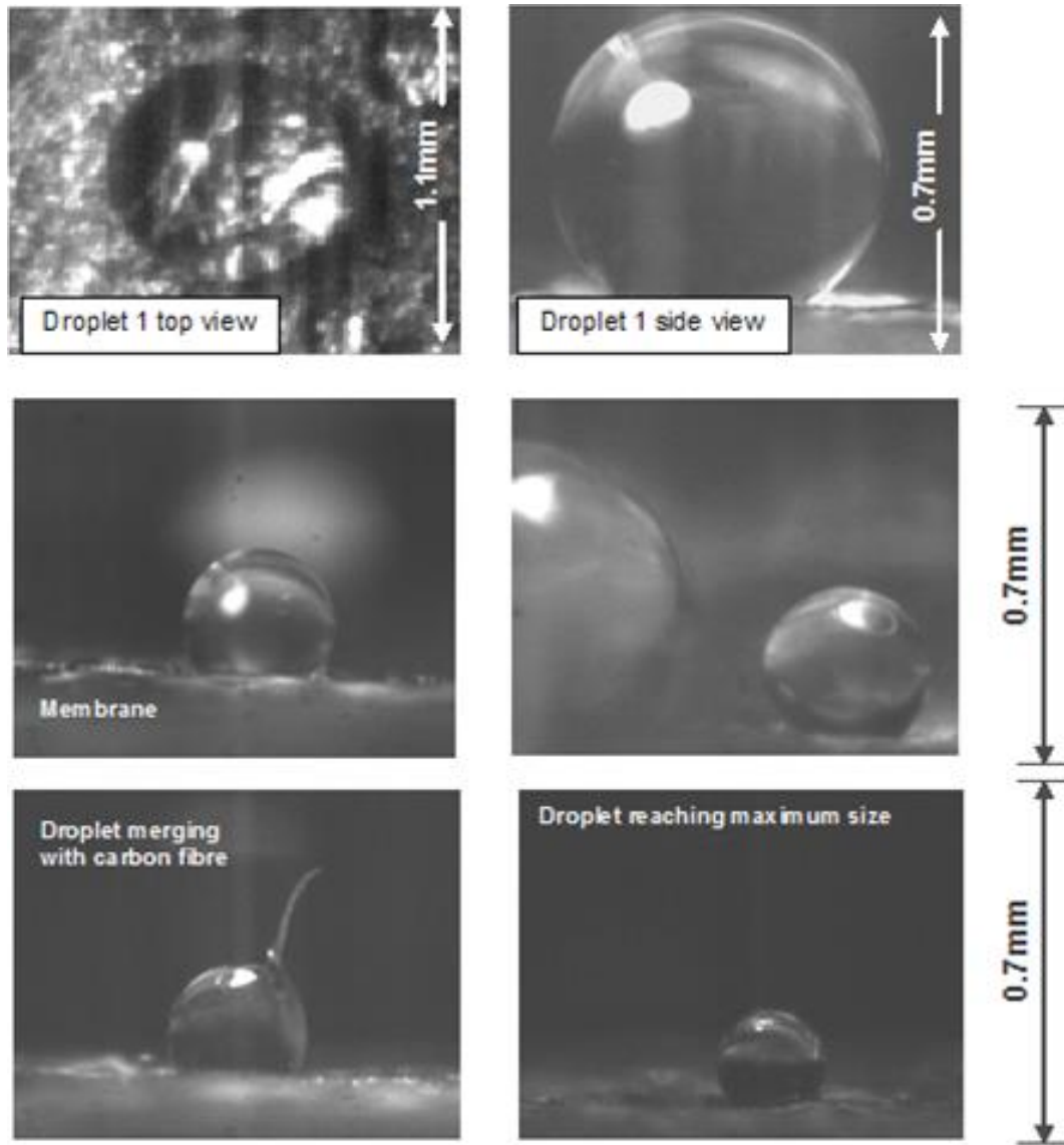
Figure 14 Droplet formation on the surface of GDL at various locations in the cathode flow channels [141]
