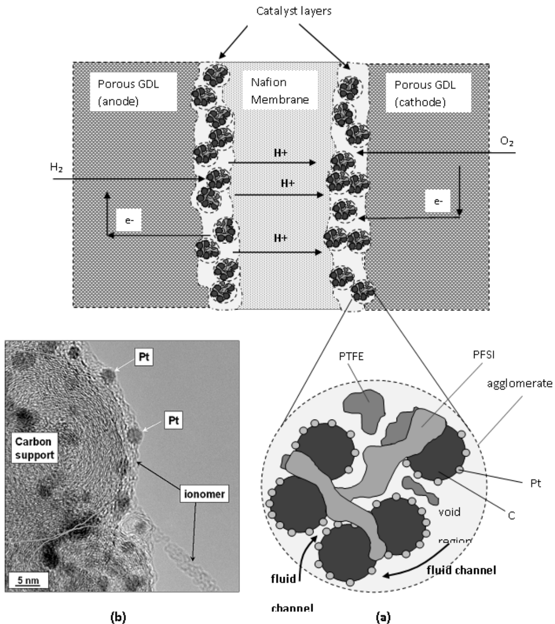
Figure 7 (a) Cross-sectional view of a typical Membrane Electrode Assembly (MEA) of PEMFC (b) TEM Image of Pt catalyst particles on carbon support surrounded by recast ionomer h (4.b is reproduced from [362] with permission)
