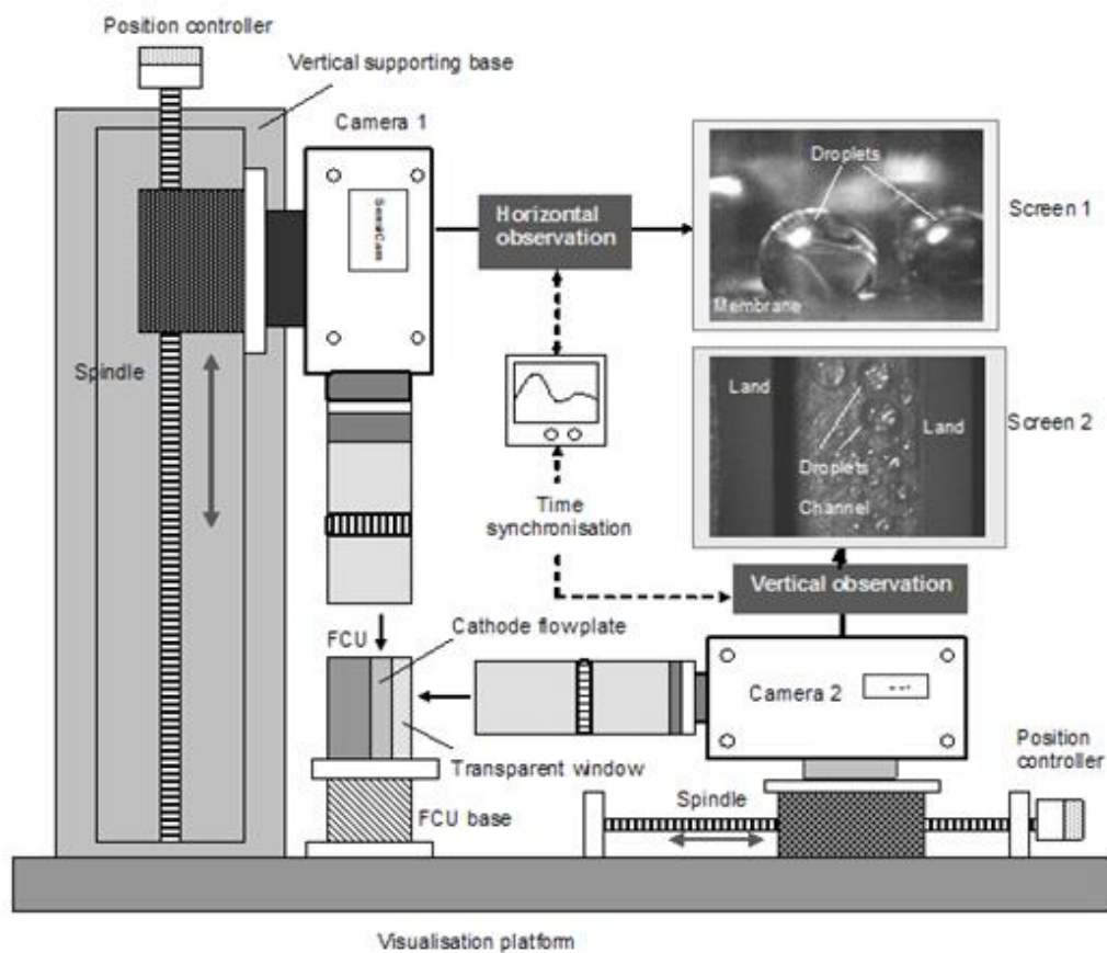
Figure 13 Visualisation set-up [141]
