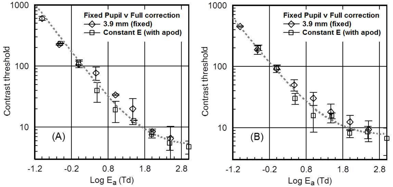
Fig. 5. Functional contrast sensitivity thresholds as a function of effective retinal illuminance measured for a Landolt ring stimulus, and plotted on a log scale at (A) the fovea and (B): \pm 5 deg in the periphery. Each graph compares thresholds measured using an unrestricted pupil size or a fixed pupil diameter of 3.9 mm. The natural pupil method employed a dynamic feedback technique to control the luminance of the screen so as to maintain the required level of retinal illuminance; both measures incorporate the Applegate apodization. The dotted line represents the function, CT = b_1 \times \text{Exp}(-b_2 \times \log(E)) + b_3 , which was fitted to the combined data sets. Fovea: b_1 = 94.71 , b_2 = -1.82 , b_3 = 5.03 ; \pm 5 deg: b_1 = 78.04 , b_2 = -1.72 , b_3 = 7.5 .
