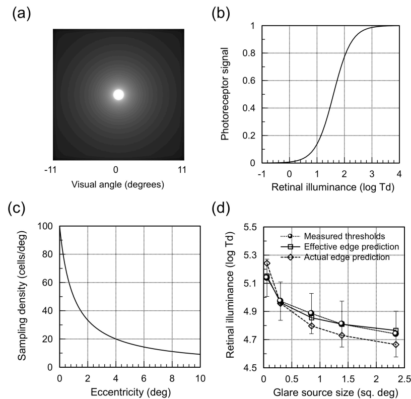
Figure 5. Discomfort glare saturation model. (a) Convolved target image with the point spread function of the eye (b) Photoreceptor response function modelled as a Michaelis-Menton function, E^n/(E^n + \delta^n) , E = retinal illuminance, \delta = 39.81 Trolands (1.6 log Trolands) represents the half response and was based on the average background retinal illuminance, n = 1.33 resulting in approximately a 3 log-unit range response. (c) Midget ganglion cell sampling density as a function of eccentricity 42 . (d) Model predictions of discomfort glare threshold as a function of source size. The blue dashed line represents the circumference of the glare source weighted by the retinal ganglion cell density. The weighting was accomplished by multiplying the circumference of each source size by its ganglion cell density at the eccentricity of its circumference; the reciprocal for each source was then scaled so that the overall mean matched that of the measured discomfort glare thresholds. The red dashed line represents the effective edge prediction: the circumference of the target in the
