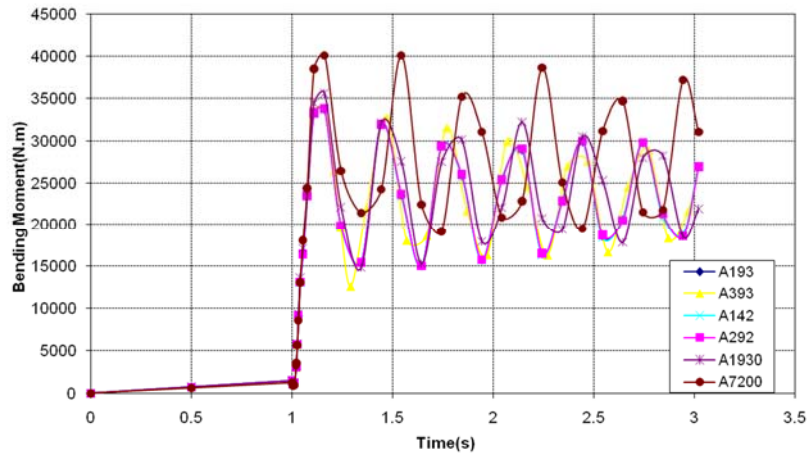
Fig.15 Major Moment at B1 of Beam A1-B1 at ground level with different mesh (1 column removal)
