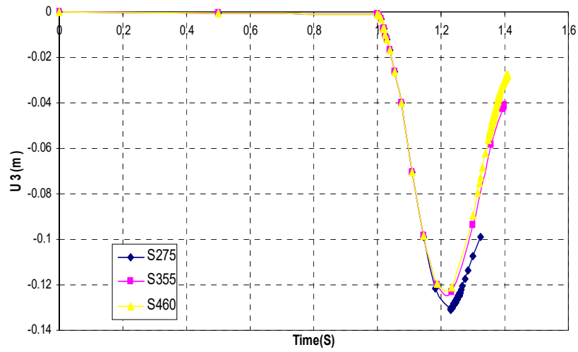
Fig.7 Displacement of the node at A1 with different steel grade of steel members (2 columns scenario)
