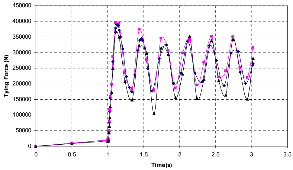
Fig.12 Tying force Beam of A1-B1 at ground level with different concrete strength (1 column removal)
