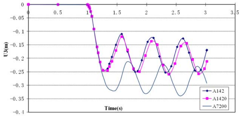
Fig. 16 Displacement of the node above the removed column with different mesh (3 columns removal)
