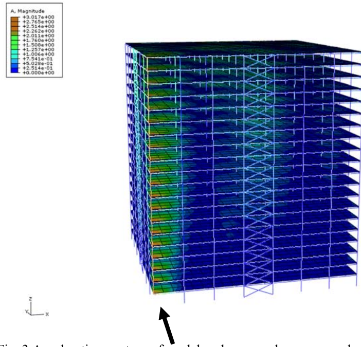
Fig .3 Acceleration contour of model under one column removal scenario
