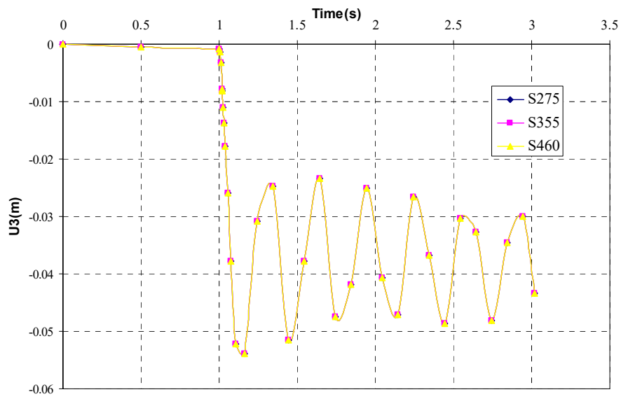
Fig.4 Displacement of the node above the removed column with different steel grade of steel members
