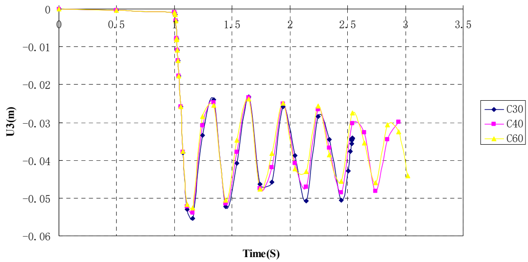
Fig.10 Displacement of the node above the removed column with different concrete strength (1 column removal)
