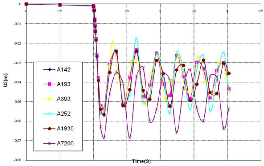
Fig. 13 Displacement of the node above the removed column with different mesh (1 column removal)
