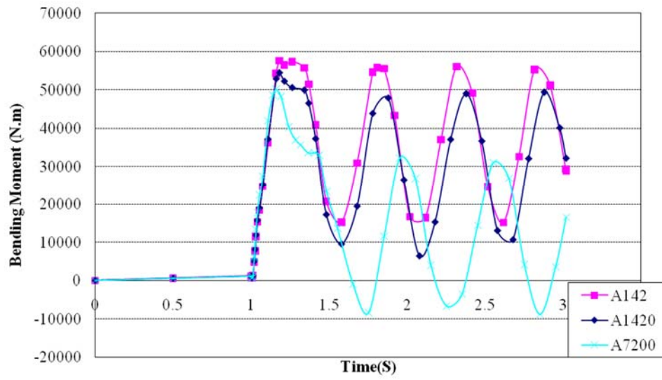
Fig.18 Major Moment at At C1 of Beam B1-C1 at ground level with different mesh (3 columns removal)
