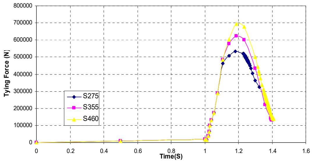
Fig.9 Tying force in the beam B1-A1 at ground level with different steel grade of steel members (2 columns scenario)
