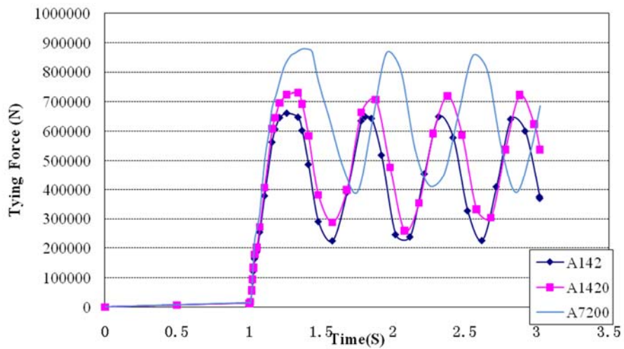
Fig.17 Axial force of At C1 of Beam B1-C1 at ground level with different mesh (3 columns removal)
