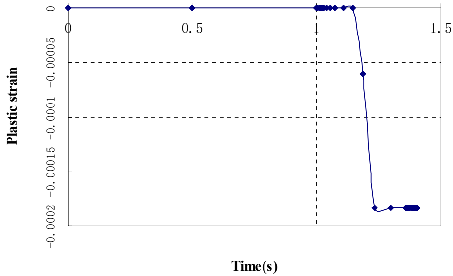
Fig.6 Axial Plastic strain of beam B1-A1 at ground level for case with S355 strength (2 columns removal)
