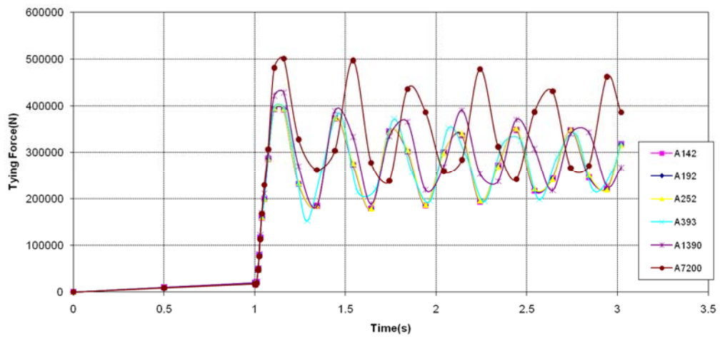
Fig.14 Axial force of At B1 of Beam A1-B1 at ground level with different mesh (1 column removal)
