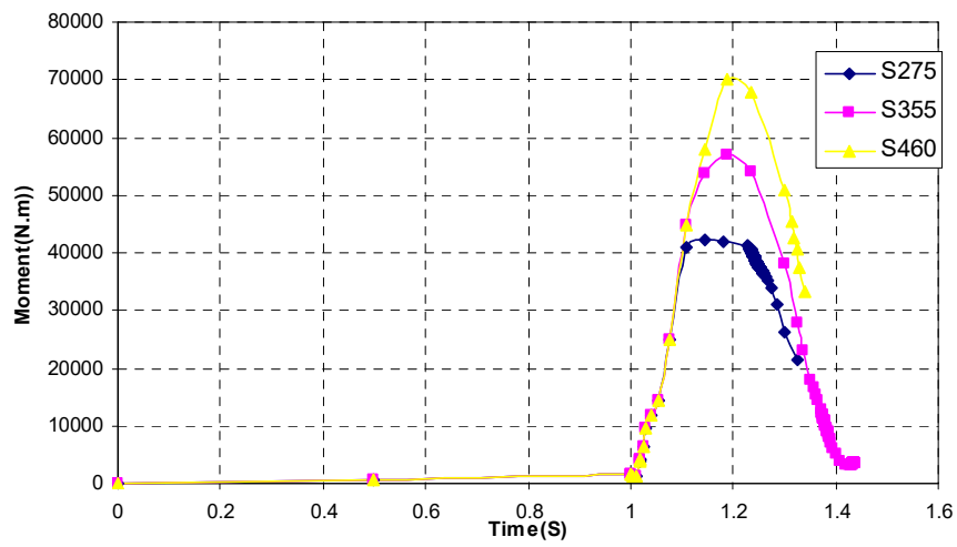
Fig.8 Major Moment of at B1 in Beam B1-A1 at ground level with different steel grade for steel member (2 columns scenario)
