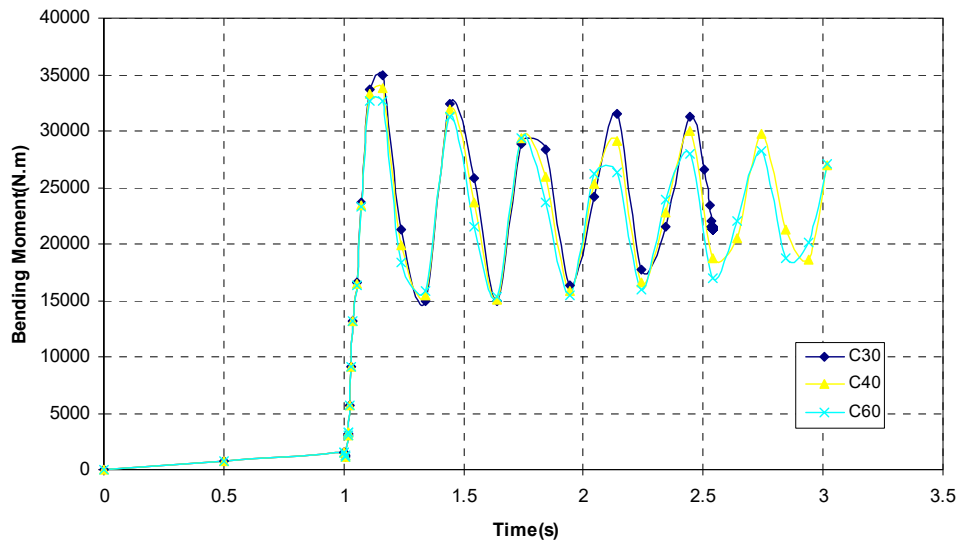
Fig.11 Major Moment of At end B1 of Beam A1-B1 at ground level with different concrete strength (1 column removal)
