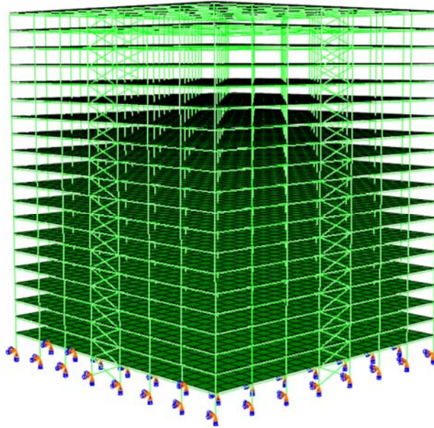
Fig 1 Analysis model with braces as lateral bracing
