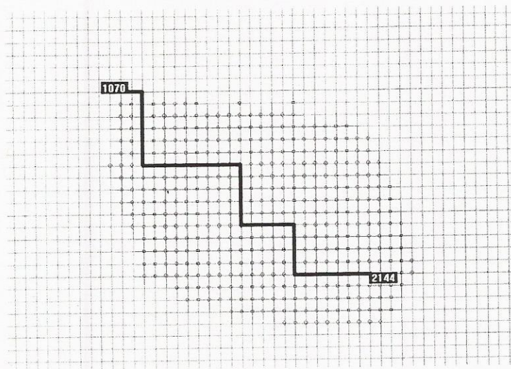
Figure 4: A* search for the normal shortest path from destination node to start node
