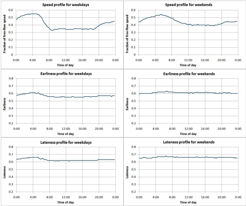
Simulated speed and reliability data: average speed, earliness and lateness profiles 400x336mm (96 x 96 DPI)
