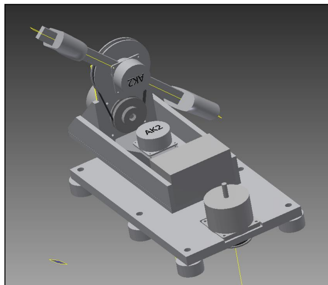
Figure 7: iBike Simulator CAD Model
