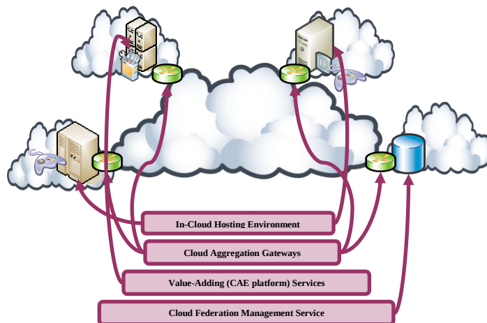
Fig. 2. The conceptual layering of the various services provided by the cloud aggregation ecosystem model.
