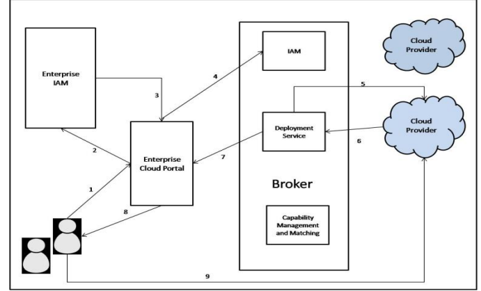
Fig. 6. Steps involved in a user creating a compute environment on a IaaS cloud service through a Broker service.
