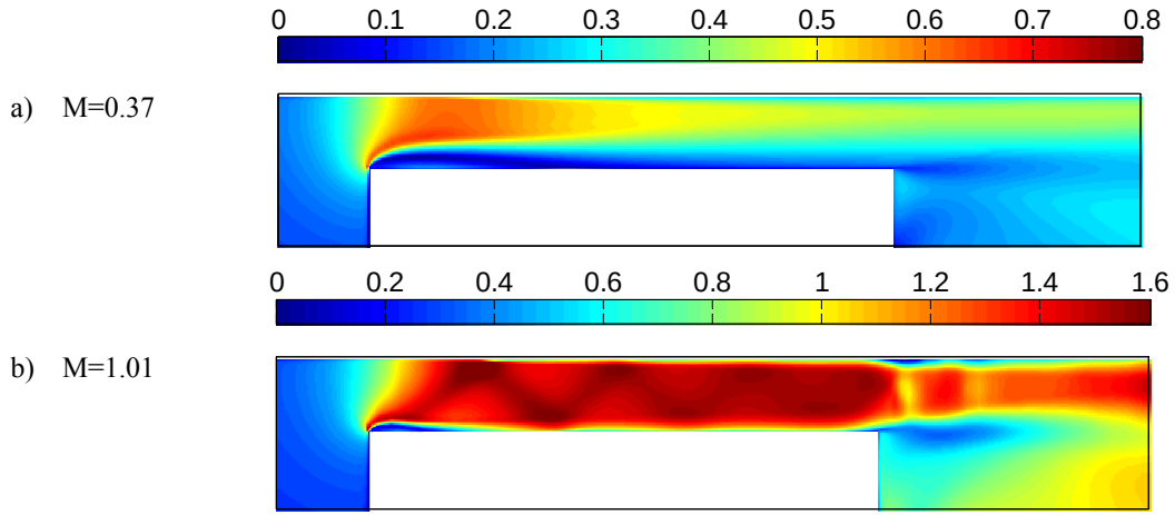
Fig. 5 Mach number contours along an axial cut plane (at x/C_x \sim 0.7 ) for subsonic and transonic tip flow.
