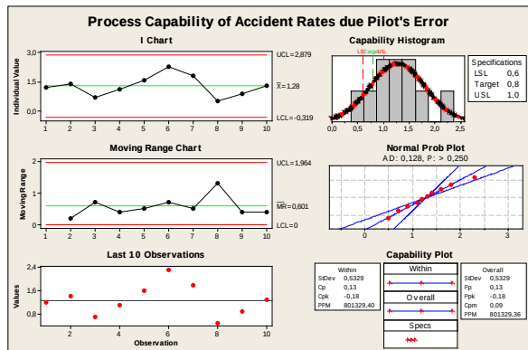
Fig. 6: Process Capability Analysis for Data
