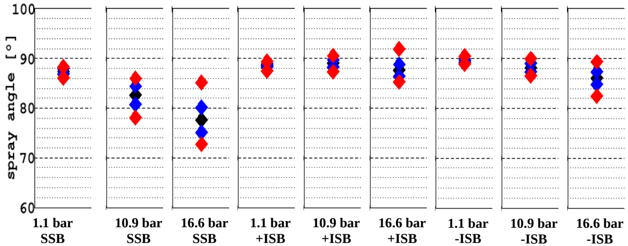
Fig. 24 Angle comparison of single injection for three prototype injectors at different backpressures, full needle lift, 1000rpm, P_i=200\text{bar} .
