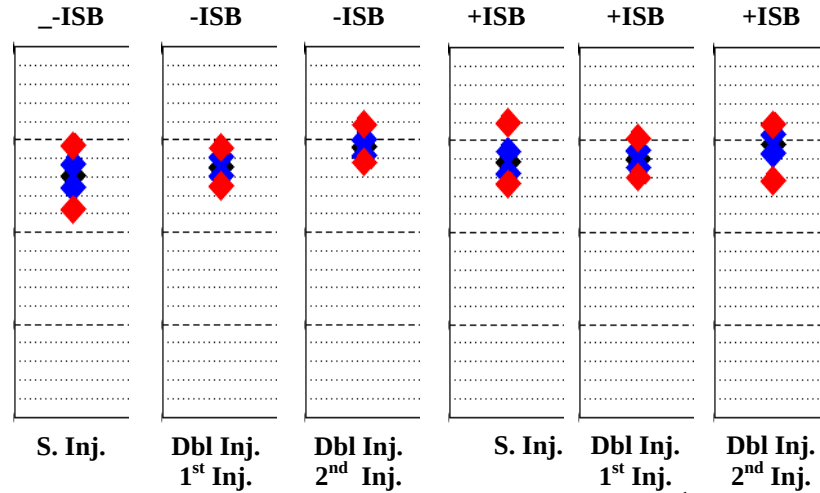
Fig. 23 Angle comparisons between single and double injection (1 st and 2 nd injection events) for ISB injectors at full lift, P_i=200\text{bar} , P_b=16.6\text{bar} .
