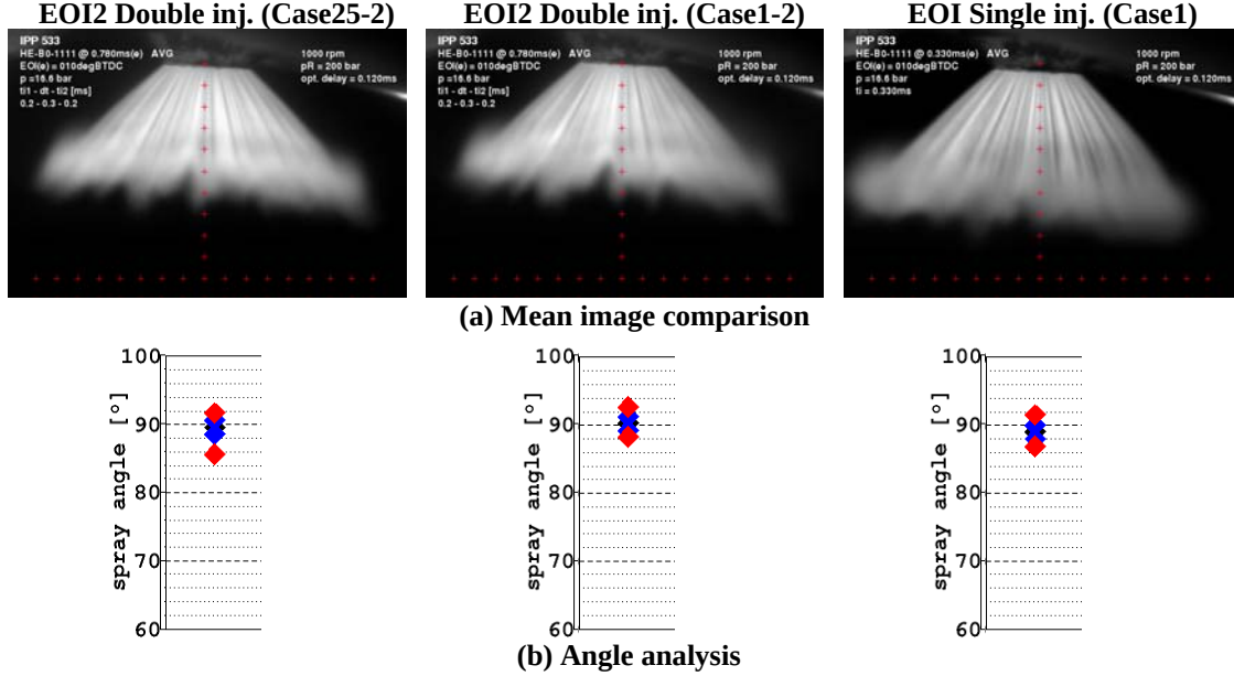
Fig. 19 Reference comparison of second injection event from +ISB injector for different test cases but at the same EOI, full needle lift, 1000rpm, P_i=200\text{bar} , P_b=16.6\text{bar} : (a) Mean image comparison; (b) Angle analysis.
