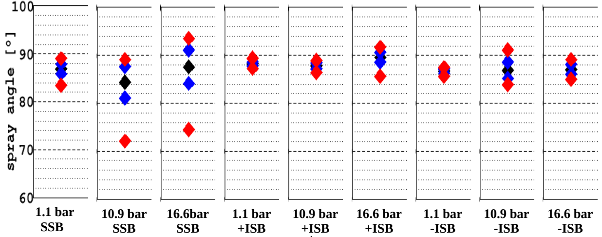
Fig. 25 Angle comparison of double injection (2 nd injection event) for three prototype injectors at different backpressures, full needle lift, 1000rpm, P_i=200\text{bar} .
