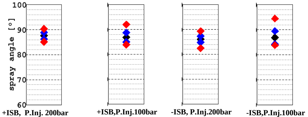
Fig. 26 Angle comparison of double injection (2 nd injection event) for two ISB prototype injectors at different injection pressure, full needle lift, 1000rpm, P_b=16.6\text{bar} .
