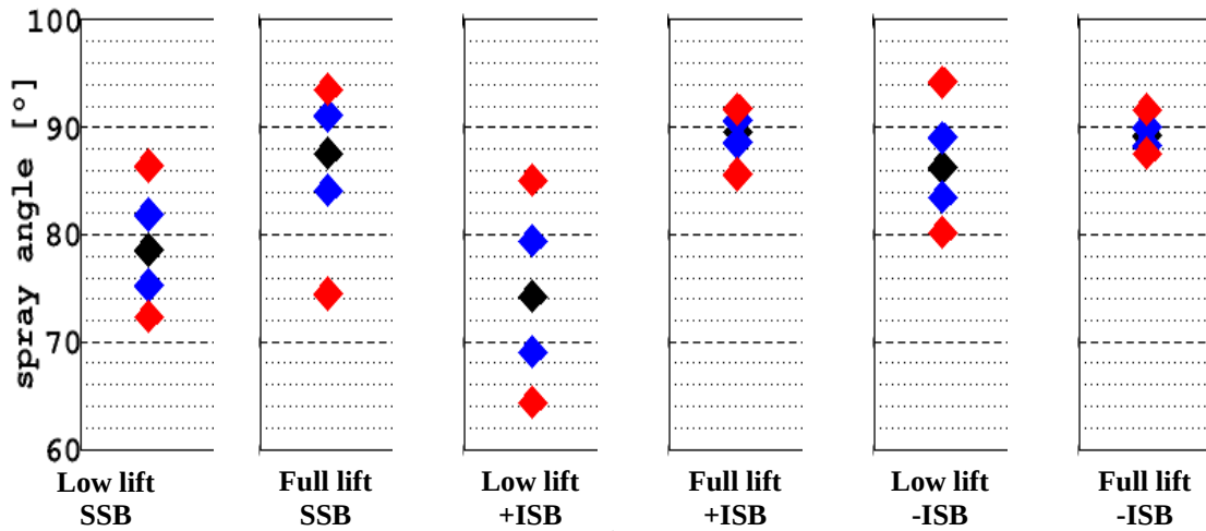
Fig. 27 Angle comparison of double injection (2 nd injection event) for two ISB prototype injectors at different needle lift, 1000rpm, P_b=16.6\text{bar} , P_i=200\text{bar} .
