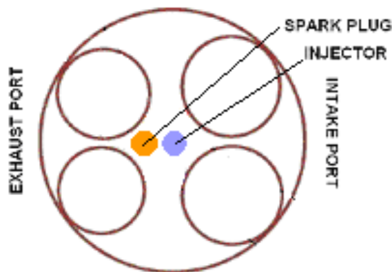
Fig. 2 Flame deck configuration of Hydra engine.
