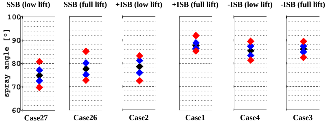
Fig. 17 Angle comparisons for different needle lifts for the three injector prototypes at 1000rpm, P_i=200\text{bar} , P_b=16.6\text{bar} .
