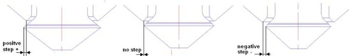
Fig. 3 Injector geometries: Inward Seal Band positive step (+ISB), Inward Seal Band negative step (-ISB) and Standard Seal Band No step (SSB).
