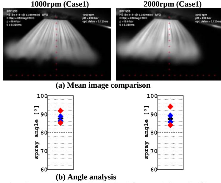
Fig. 13 Effect of engine speed on spray from +ISB injector at full needle lift, P_b=16.6\text{bar} , P_i=200\text{bar} : (a) Mean image comparison; (b) Angle analysis.
