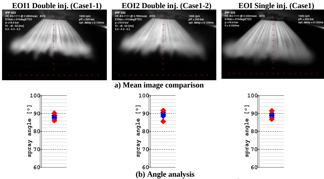
Fig. 20 Comparison between the EOI of double injection (1 st and 2 nd injection events) and single injection for +ISB injector at full needle lift, P_b=16.6\text{bar} , 1000rpm, P_i=200\text{bar} : (a) Mean image comparison; (b) Angle analysis.
