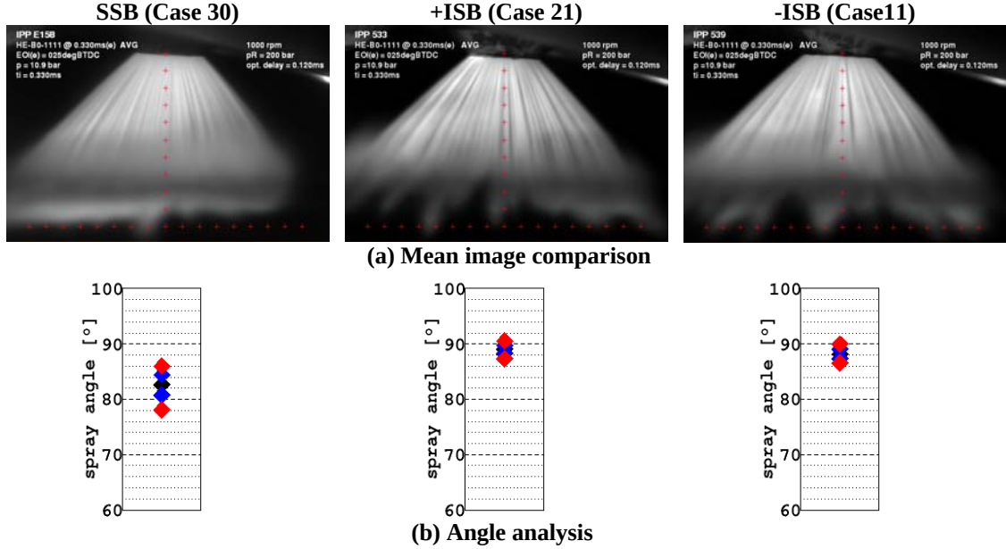
Fig. 10 Comparison between the three different injectors at full needle lift, 1000rpm, P_b=10.9\text{bar} , P_i=200\text{bar} : (a) Mean image comparison; (b) Angle analysis.
