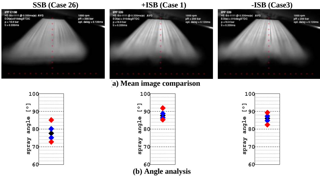
Fig. 11 Comparison between the three different injectors at full needle lift, 1000rpm, P_b=16.6\text{bar} , P_i=200\text{bar} : (a) Mean image comparison; (b) Angle analysis.
