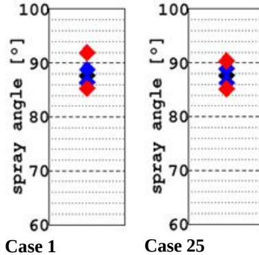
Fig. 7 Statistical angle comparison for the same operating condition. (Case 1 and Case 25)
