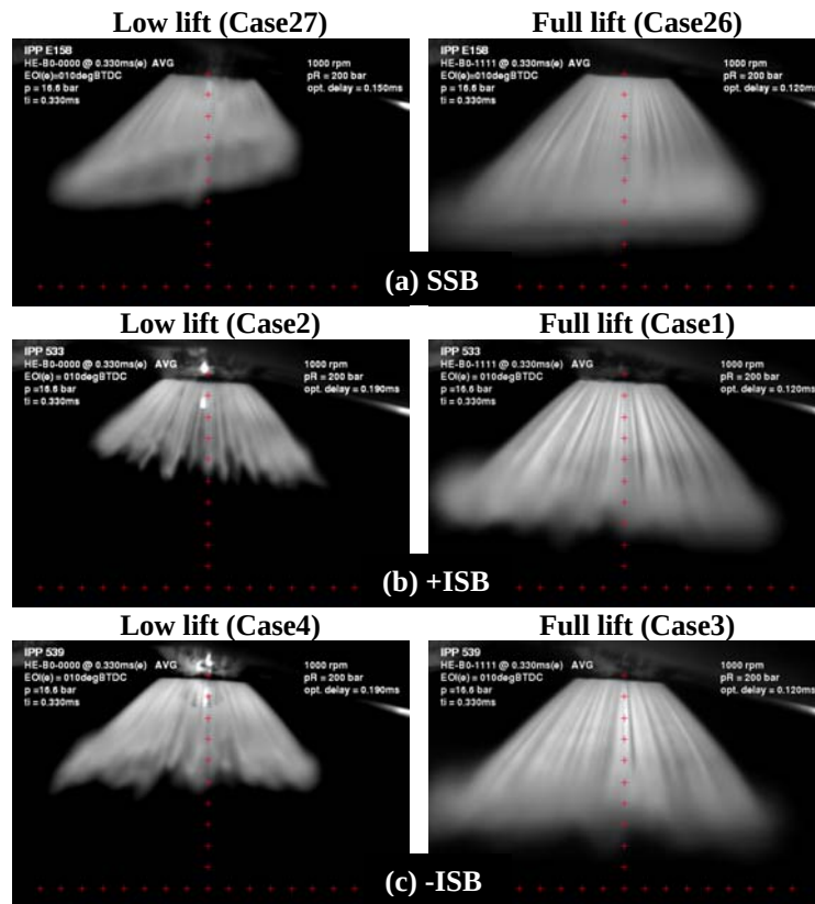
Fig. 16 Mean spray image comparison of three prototype injectors at low (left column) and full (right column) needle lifts, P_b=16.6\text{bar} , 1000\text{rpm} , P_i=200\text{bar} : (a) SSB prototype; (b) +ISB prototype; (b) -ISB prototype.
