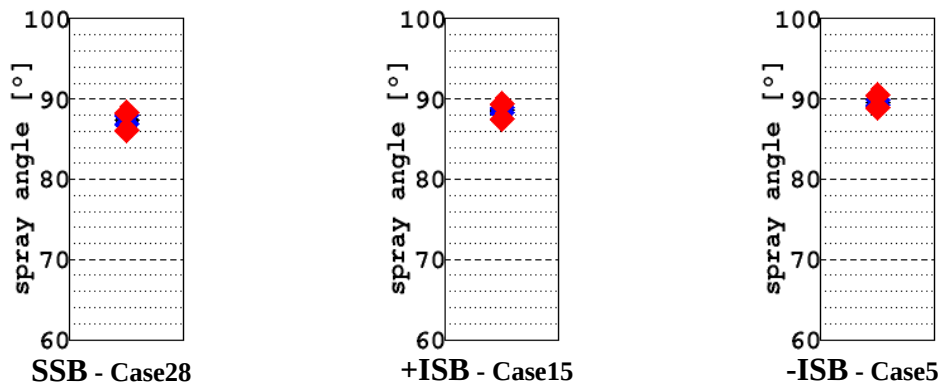
Fig. 9 Angle comparison for three different injector prototypes: Full needle lift, 1000rpm, P_b=1.1\text{bar} , P_i=200\text{bar} .
