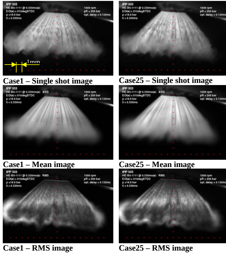
Fig. 6 Reference comparison of single shot, mean and RMS spray images for the same operating condition. (Case 1 vs Case 25)
