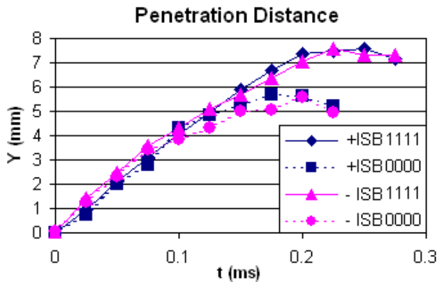
Fig. 18 Spray tip penetration as a function of time after SOI at full and low needle lifts for ISB injectors: 1000rpm, P_i=200\text{bar} , P_b=16.6\text{bar} .
