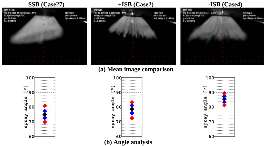
Fig. 12 Comparison between the three different injectors at low needle lift, 1000rpm, P_b=16.6\text{bar} , P_i=200\text{bar} : (a) Mean image comparison; (b) Angle analysis.
