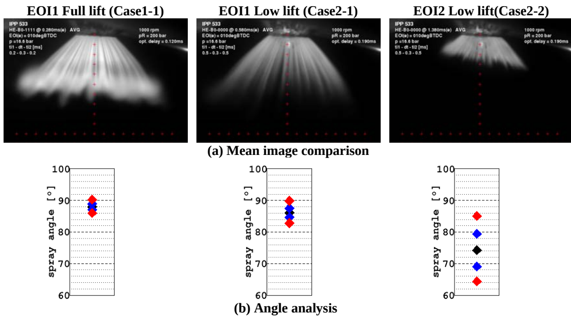
Fig. 21 Effect of needle lift on double injection sprays for +ISB injector and at different EOIs, P_b=16.6\text{bar} , 1000\text{rpm} , P_i=200\text{bar} : (a) Mean image comparison; (b) Angle analysis.
