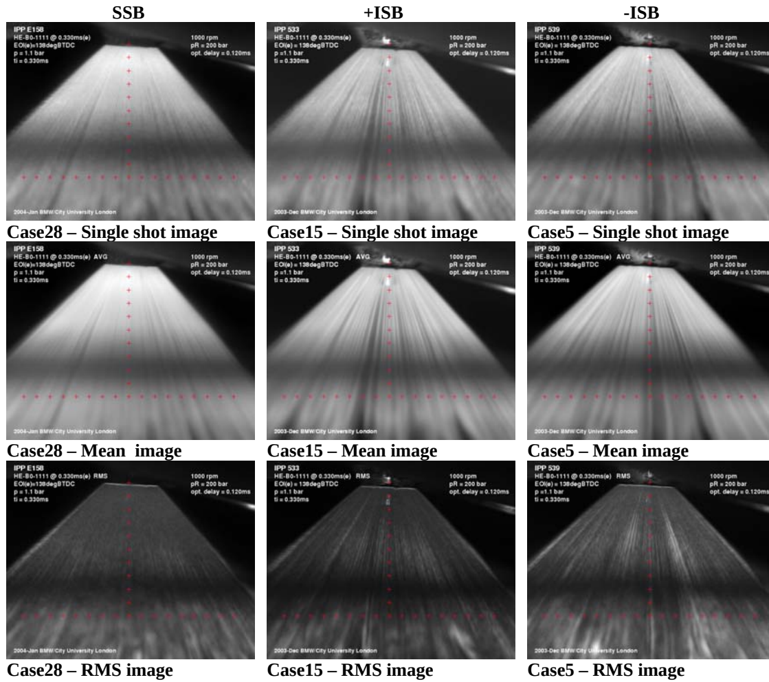
Fig. 8 Image comparison for three different injector prototypes: Full needle lift, 1000rpm, P_b=1.1\text{bar} , P_i=200\text{bar} .
