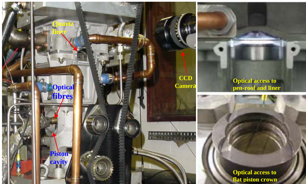
Fig. 1 Model Hydra optical engine with limited quartz window.
