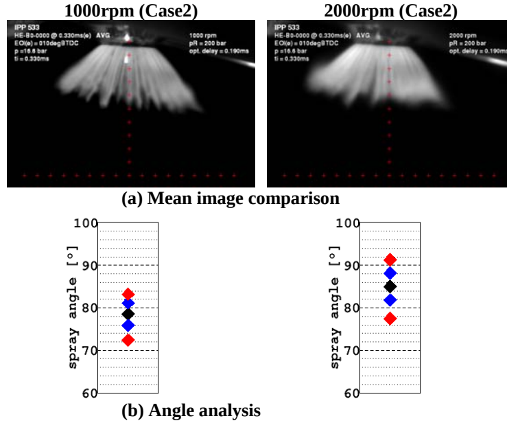
Fig. 14 Effect of engine speed on spray from +ISB injector at low needle lift, P_b=16.6\text{bar} , P_i=200\text{bar} : (a) Mean image comparison; (b) Angle analysis.
