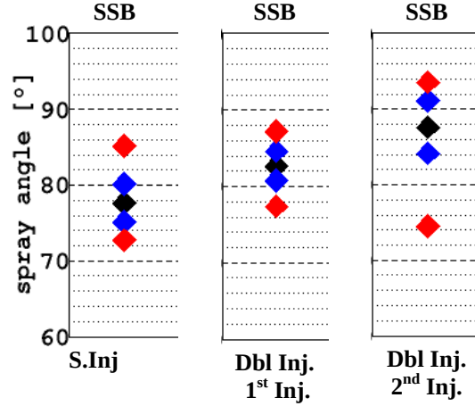
Fig. 22 Angle comparisons between single and double injection (1 st and 2 nd injection events) for SSB injector at full lift, P_i=200\text{bar} , P_b=16.6\text{bar} .
