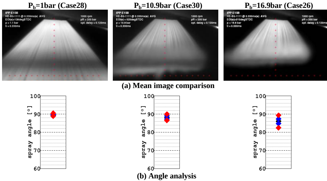
Fig. 15 Effect of cylinder back pressure on spray from SSB injector at full needle lift, 1000rpm, P_i=200\text{bar} : (a) Mean image comparison; (b) Angle analysis.
