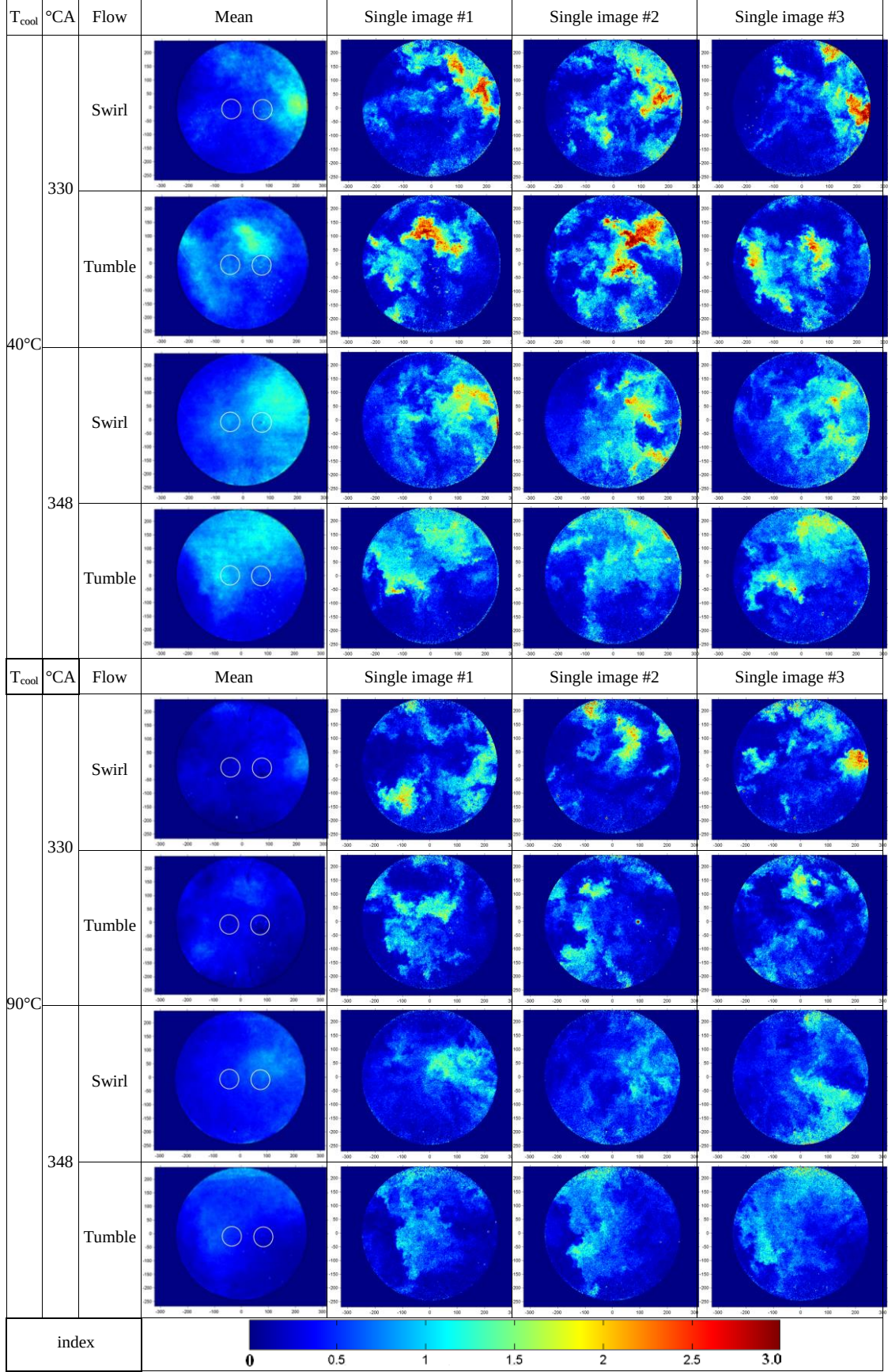
Figure 9 LIF images during compression stroke at p_{inj.}=120bar .
