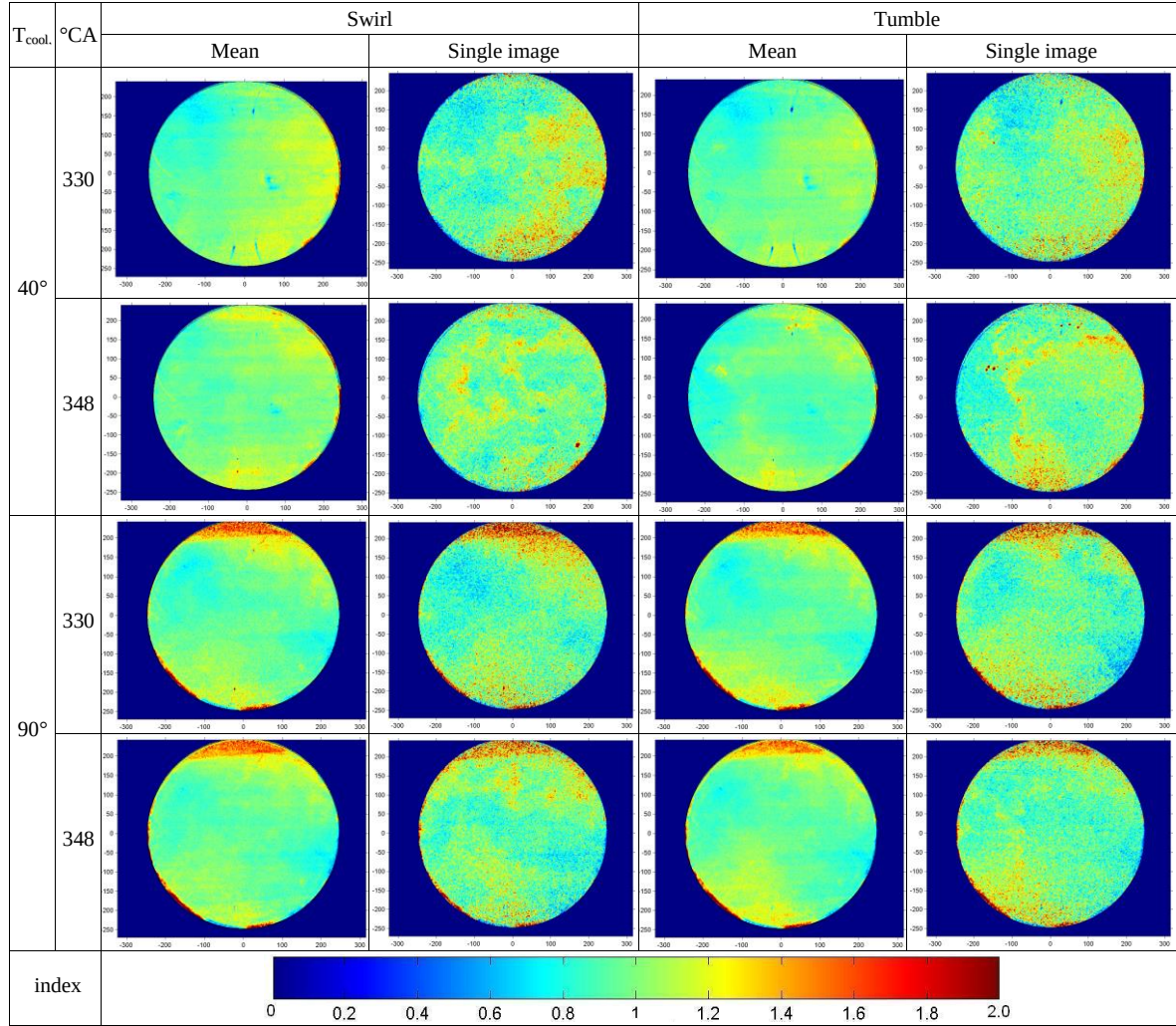
Figure 6 LIF images at 2mm below cylinder head gasket, p_{inj.} = 70\text{bar} .
