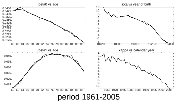
Fig 3. E&W male mortality experience, ages 60-89. APC back-fitting exercise. Reduction factor parameter estimates, with beta parameter smoothing.
