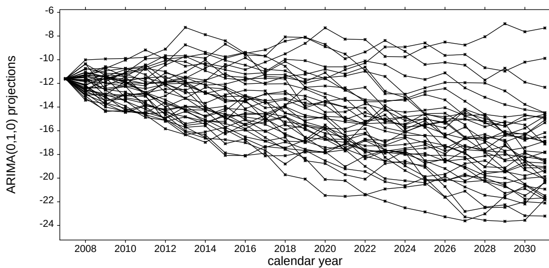
Algorithm 2 (without Step 1): 40 simulations
