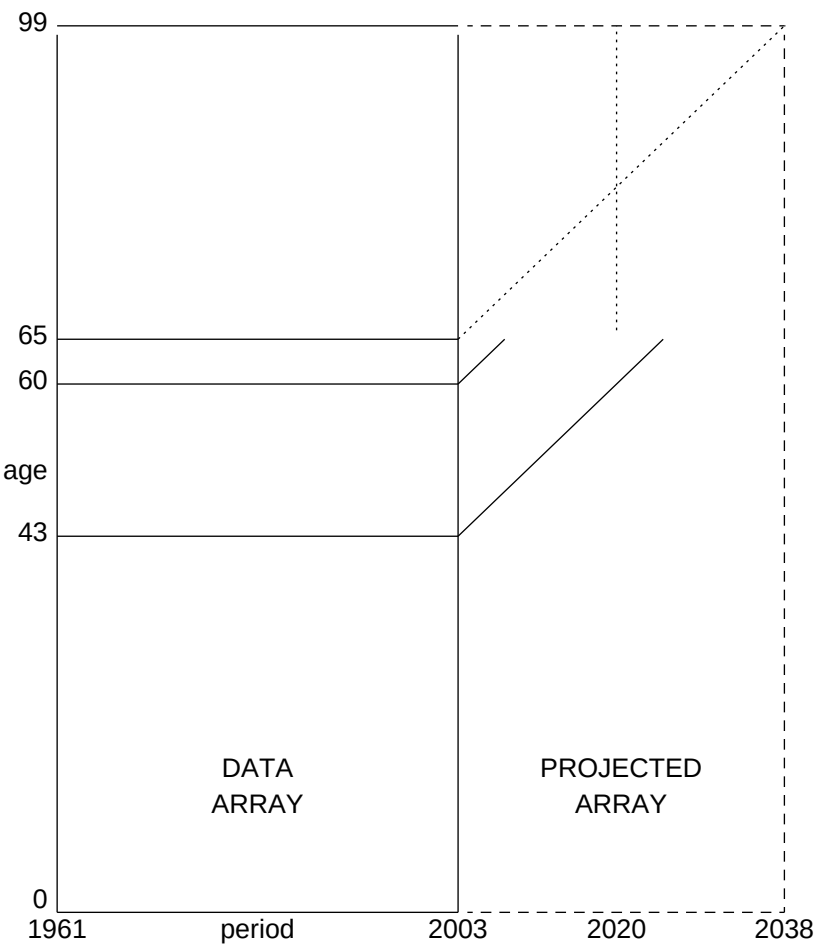
Fig 2. England & Wales 1961-2003 male mortality experience, ages 0-99. Schematic data and projected arrays highlighting projected trajectories (dotted lines) needed when computing statistics of interest (a) by cohort for an individual aged 65 in year 2003, and (b) by period for an individual aged 65 in year 2020. This implies retaining data aged 60 and above for (a), and data aged 43 and above for (b): allowing for the zero weighting of the 5 most recent cohorts in the resulting data array, when truncated. However, truncation by age, involves discarding data contributing directly to relevant cohorts: bounded by the back projection of the (thick) diagonal lines in the projected array.
