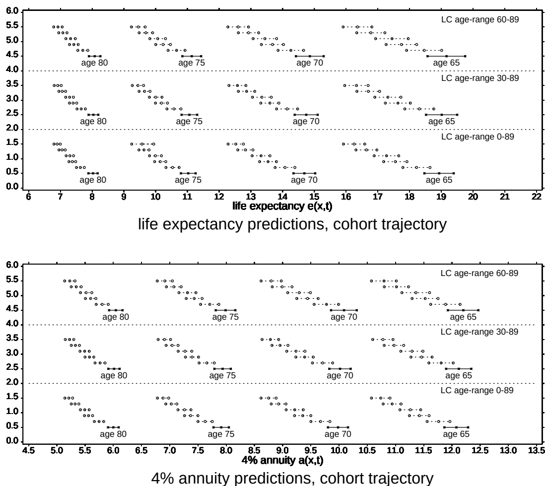
Fig 13. E&W male mortality experience, ages 60-89; 30-89; 0-89. LC model. Evolving biennial (1997, 99, 01, 03, 05, 2007) life expectancy and 4% fixed rate annuity predictions, by cohort trajectory: presented in decreasing sequence, for individuals aged 65, 70, 75, 80 respectively. Prediction intervals by bootstrapping the time series prediction error and selecting 2.5, 50, 97.5 percentiles.
