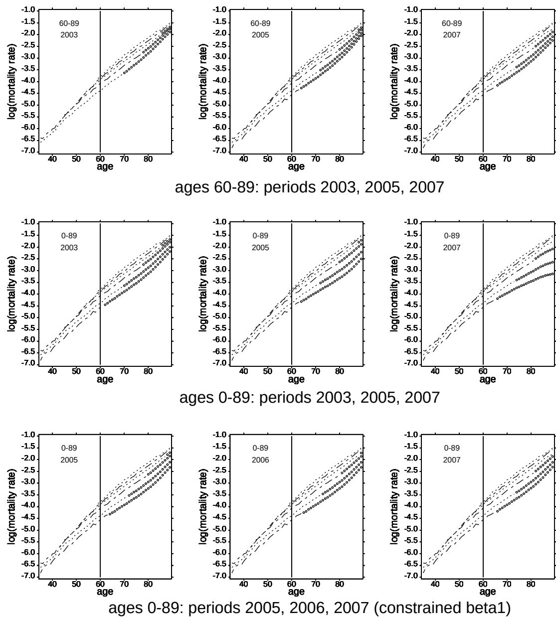
Fig 9. E&W male mortality experience. Empirical log mortality rate profiles with APC forecasts, by individual cohort year-of-birth: 1902, 1910, 1918, 1926, 1934, 1942.
