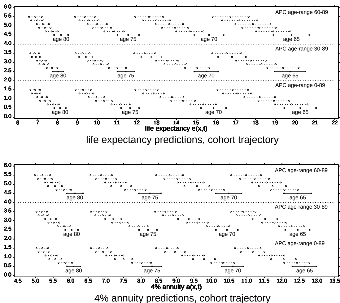
Fig 10. E&W male mortality experience, ages 60-89; 30-89; 0-89. APC model. Evolving biennial (1997, 99, 01, 03, 05, 2007) life expectancy and 4% fixed rate annuity predictions, by cohort trajectory: presented in decreasing sequence, for individuals aged 65, 70, 75, 80 respectively. Prediction intervals by bootstrapping the time series prediction error and selecting 2.5, 50, 97.5 percentiles.
