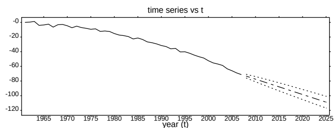
Fig 12. E&W male mortality experience. LC model: period index time series (modelled post 1978), two cases. First row: R^2 linear regression goodness-of-fit statistic. Second row: ARIMA(1,1,0) time series residuals. Third row: full time series with predictions and prediction intervals.
