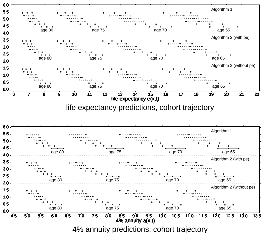
Fig 14. E&W male mortality experience, ages 60-89. APC modelling. Evolving biennial (1997, 99, 01, 03, 05, 2007) life expectancy and 4% fixed rate annuity predictions, by cohort trajectory: presented in decreasing sequence, for individuals aged 65, 70, 75, 80 respectively. Prediction intervals by simulation and selecting 2.5, 50, 97.5 percentiles using Algorithm 1 and Algorithm 2, with and without allowance for time series parameter error (pe).
