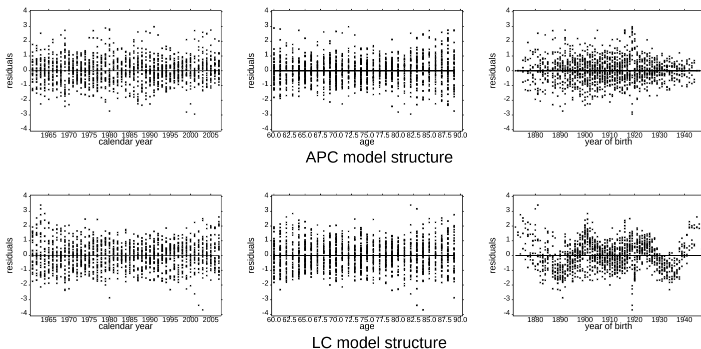
Fig 7. England & Wales 1961-2007 male mortality experience, ages 60-89. Deviance residual plots against: (i) period (left column), (ii) age (centre column), (iii) cohort year-of-birth (right column).
