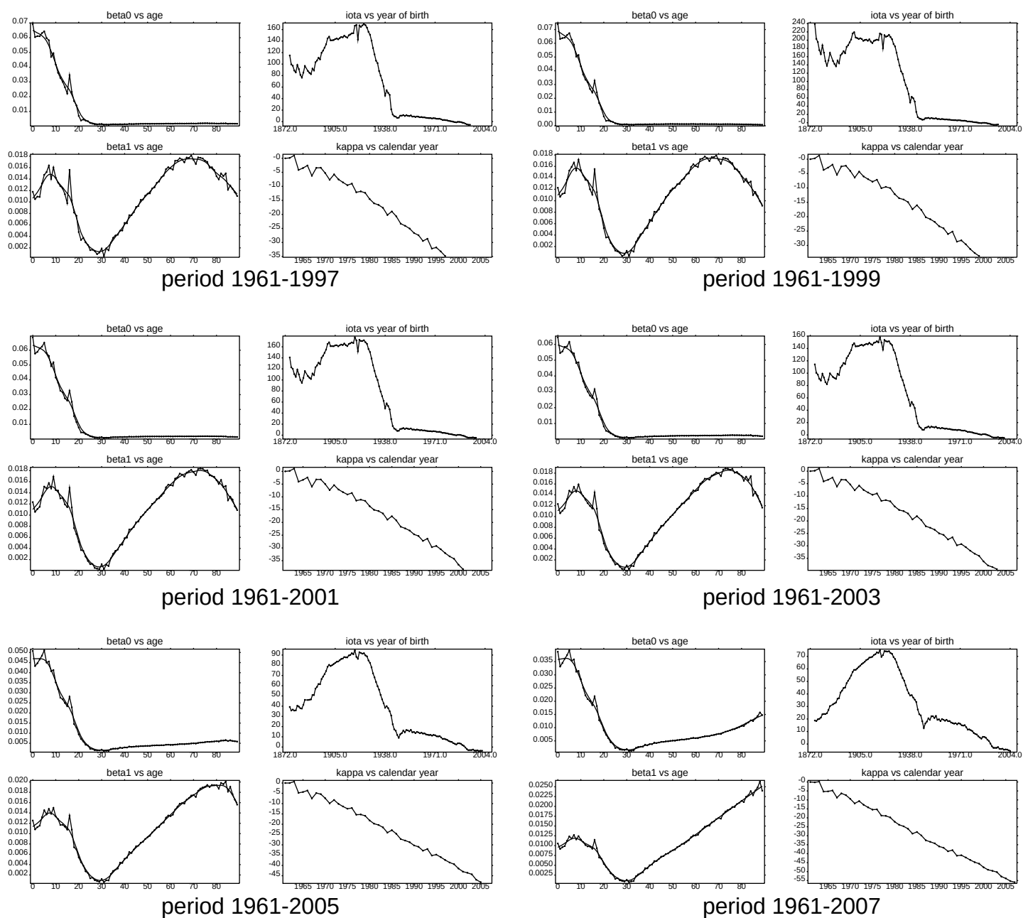
Fig 4. E&W male mortality experience, ages 0-89. APC back-fitting exercise. Reduction factor parameter patterns, with beta parameter smoothing.
