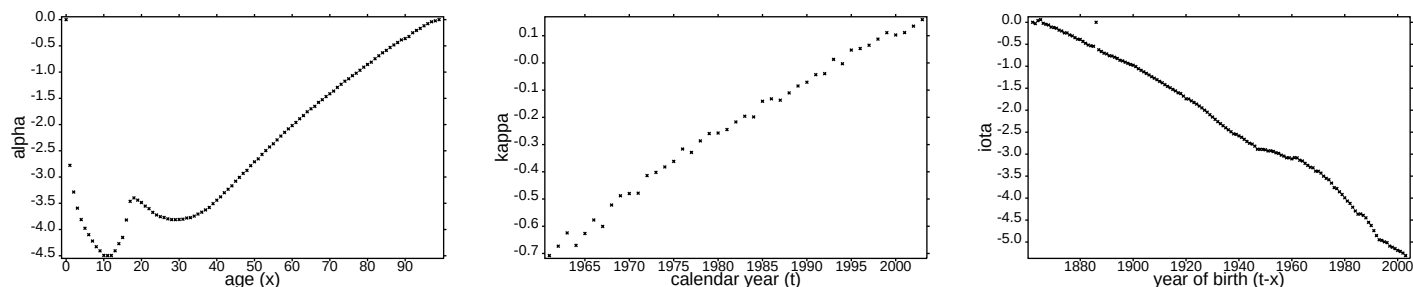
(iii) H_0: \log\{\mu(x,t)\} = \kappa(t) + \iota(t-x) + \alpha(x)
