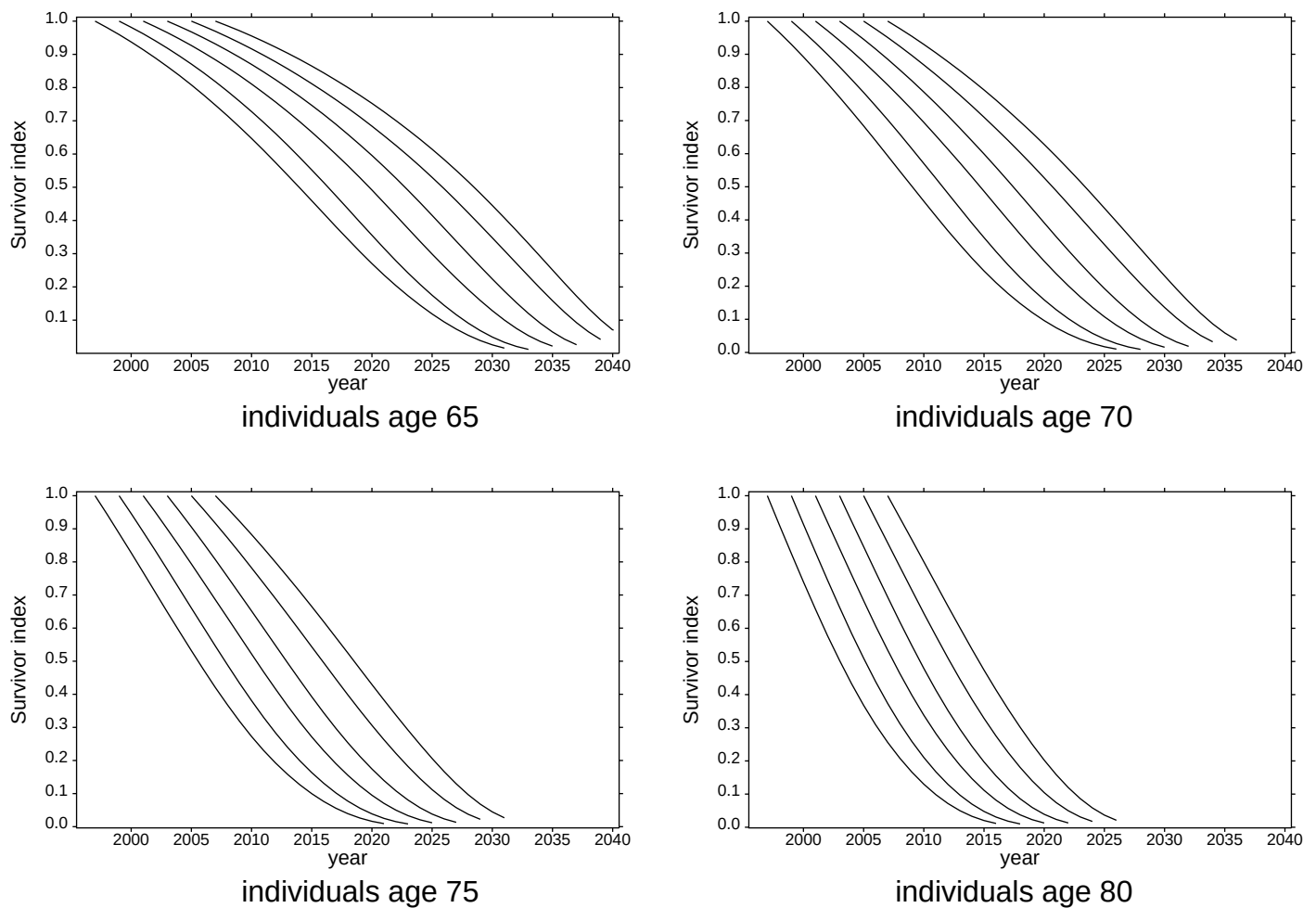
Fig 11. E&W male mortality experience (ages 0-89). APC model (with beta1 constrained post 2004). Evolving predicted survivor indices by back-fitting based on the retention of periods 1961 to 1997, 1999, 2001, 2003, 2005, 2007 respectively, depicted in sequence (within each frame): for individuals aged 65, 70, 75, 80. Simulated prediction intervals omitted.
