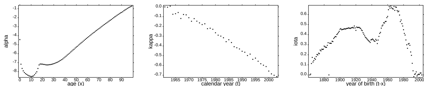
(i) H_0: \log\{\mu(x,t)\} = \alpha(x) + \kappa(t) + \iota(t-x)
