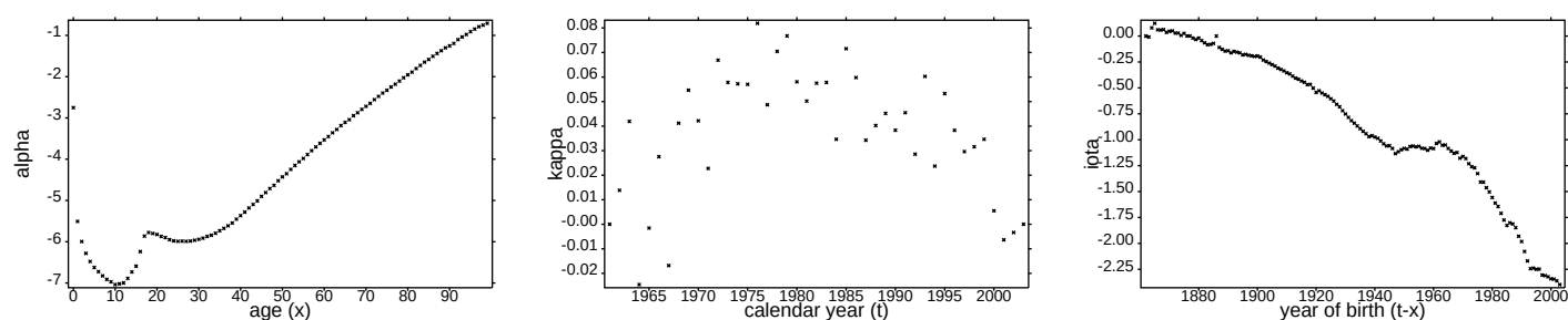
(ii) H_0: \log\{\mu(x,t)\} = \alpha(x) + \iota(t-x) + \kappa(t)
