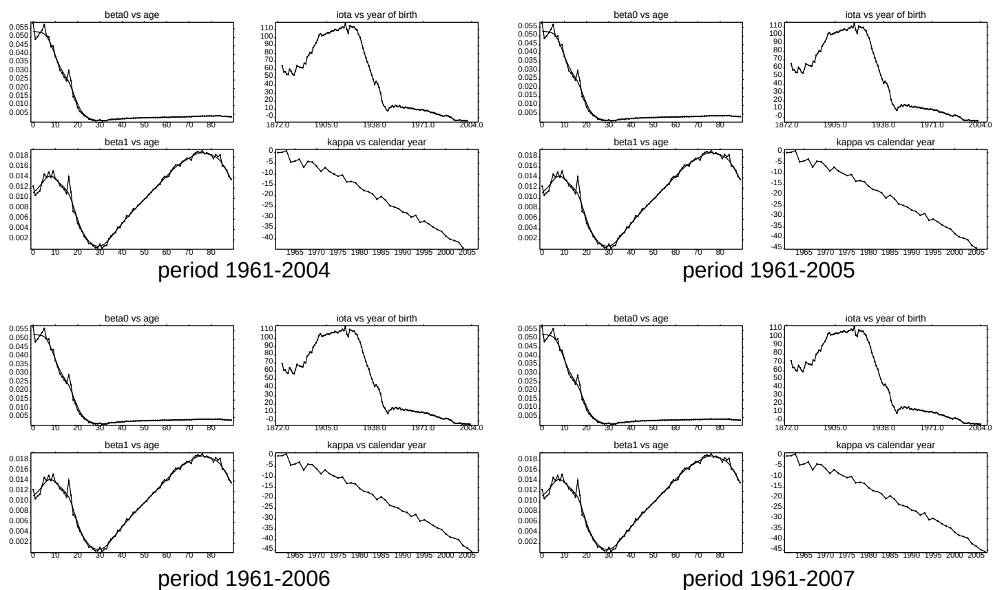
Fig 5. E&W male mortality experience, ages 0-89. APC back-fitting exercise. Reduction factor parameter patterns, with beta parameter smoothing. Patterns in the upper right, and two lower quadrants, are generated by constraining beta1 to the 1961-2004 generated pattern, depicted in the upper left quadrant.
