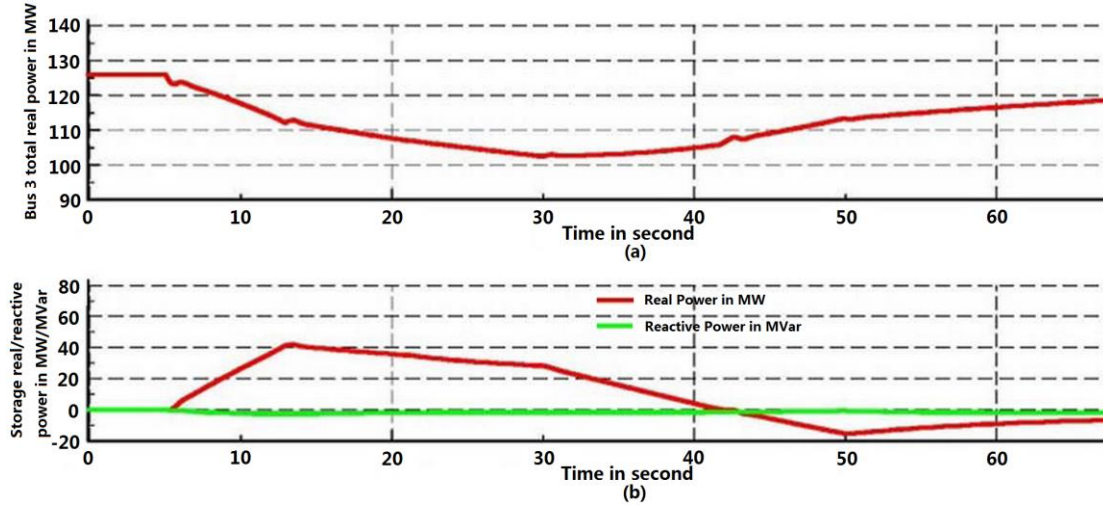
Fig. 6.15 Total active power and battery storage variation in Bus 3 when solar radiation is changing
