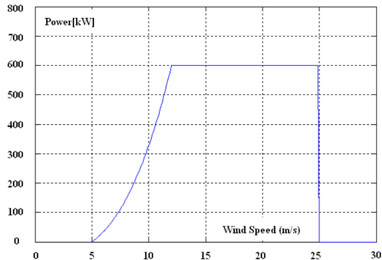
Fig. 6.9 Wind speed VS output power curve
