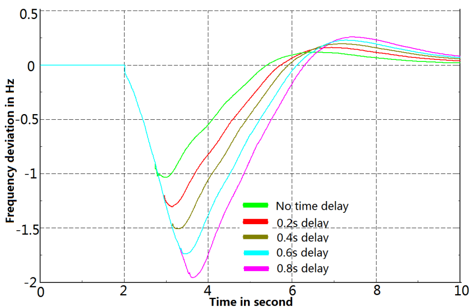
Fig. 5.11 Frequency deviation with different time delay when one step load shed is tripped at 49 Hz
