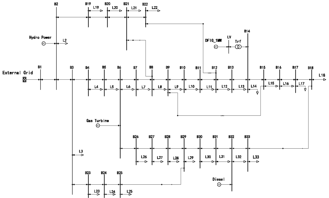
Fig. 5.9 IEEE 33-bus distribution system configuration
