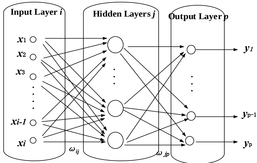
Fig. 4.10 Three-layer Network
