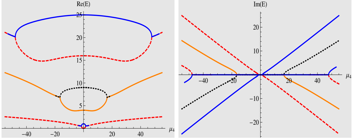
Figure 3.6: Energy eigenvalue spectra in the spontaneously broken regime for the parameter choice (3.81) as a function of \mu_4 with even (blue and orange, solid lines) and odd (black and red, dashed lines) eigenfunctions for bosonic boundary conditions. The exceptional points are located at (\mu_4 = \pm 1.4687, E = 0.5205) , (\mu_4 = \pm 16.47116, E = 6.8323) and (\mu_4 = \pm 47.80596, E = 20.1677) .
