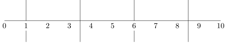
Figure 2.4: The action of W_2^5 on \Lambda_{TL_{21}} .
