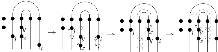
Figure 3.11: An example of move (M3).
