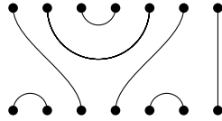
Figure 2.1: A (7, 7) -Temperley-Lieb diagram.
