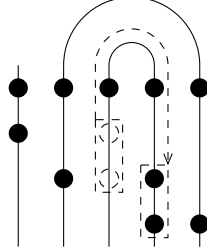
Figure 3.10: An example of move (M2).
