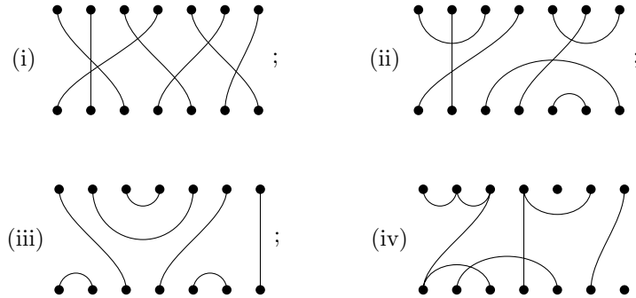
Figure 3: An example of a diagram in: (i) the symmetric group; (ii) the Brauer algebra; (iii) the Temperley-Lieb algebra; and (iv) the partition algebra.
