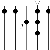
Figure 4.12: An abacus requiring moves relating to the symmetric group.
