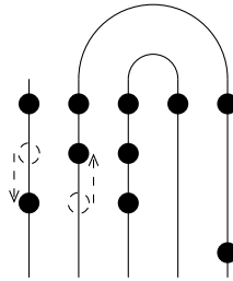
Figure 3.9: An example of move (M1).
