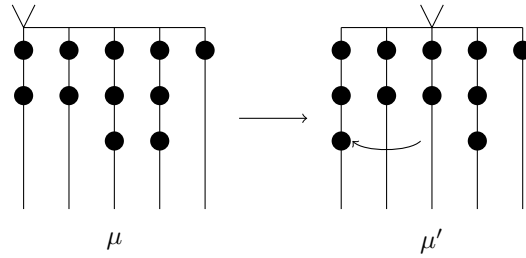
Figure 4.8: Constructing the marked abacus of \mu' from \mu .
