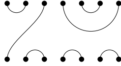
Figure 2.3: An example of a diagram in I(7, 1) .
