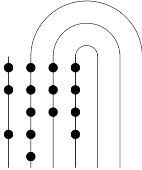
Figure 3.8: An example of a reduced linked abacus.
