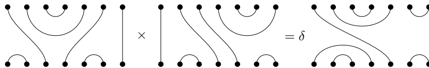
Figure 2.2: Multiplication of two diagrams in TL_7^R(\delta) .
