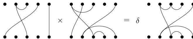
Figure 4.1: Multiplication of two diagrams in P_5^R(\delta) .
