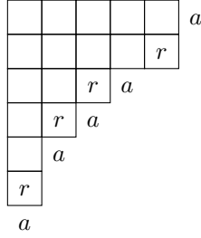
Figure 1.1: The Young diagram of \lambda = (5^2, 3, 2, 1^2) . Removable nodes are marked by r and addable nodes by a .
