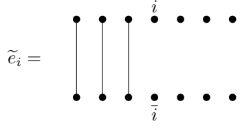
Figure 4.15: The quasi-idempotent \tilde{e}_i .
