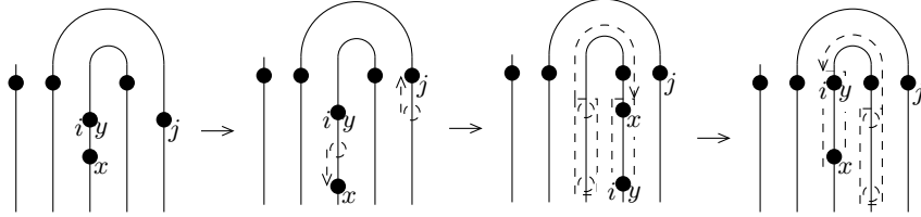
Figure 3.12: An example of move (M3) with beads i and y equal. Note that in step 2 the bead i = y does not move.
