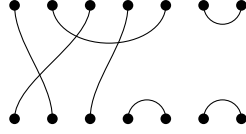
Figure 3.4: An example of diagram in I(7, 3) .
