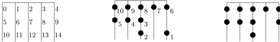
Figure 1.4: The positions on the abacus with 5 runners, the arrangement of beads (numbered) representing \lambda = (5, 4) , and the corresponding 5-core.
