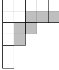
Figure 1.3: The rim hook corresponding to h_{(2,2)} . The node (2, 2) has moved to the rim.
