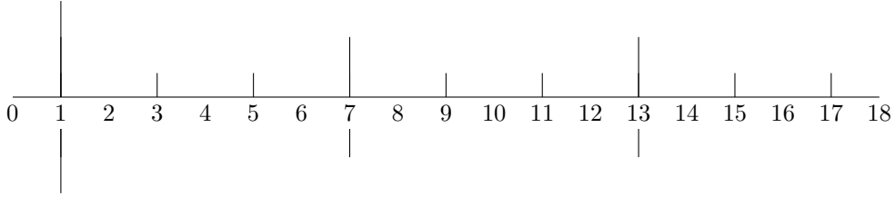
Figure 2.6: The action of W_2^4 on \Lambda_{TL_{37}} in positive characteristic.
