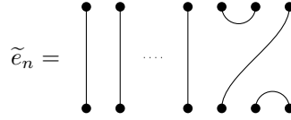
Figure 3.19: The idempotent \tilde{e}_n .
