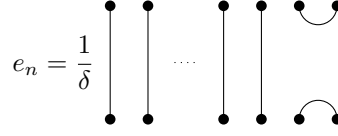
Figure 3.3: The idempotent e_n .
