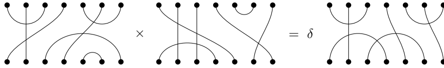
Figure 3.2: Multiplication of two diagrams in B_7^R(\delta) .
