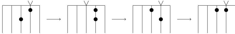
Figure 4.13: The movement of beads in Case 3'.
