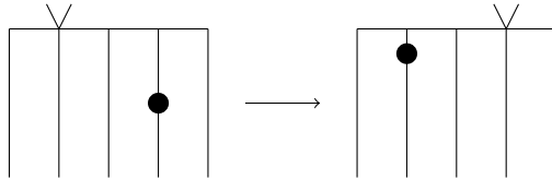
Figure 4.10: The movement of beads in Case 2.
