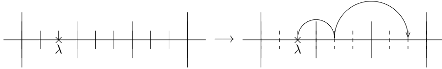
Figure 2.7: The process of the proof of Corollary 2.13. We ignore all reflections through dashed walls.
