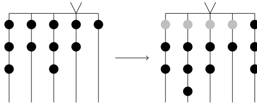
Figure 4.7: Adding 4 beads (coloured grey) to the abacus of \lambda_{\mathcal{O}} = (2, 1) . Each existing bead (coloured black) and the \vee is moved 4 places to the right.
