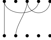
Figure 4.4: An example of a diagram in I(5, 2) .
