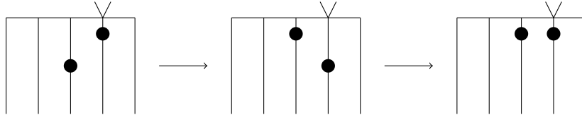
Figure 4.11: The movement of beads in Case 3.
