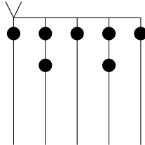
Figure 4.6: The \delta -marked abacus of \lambda , with \lambda = (2, 1) and b = 7 .
