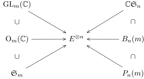
Figure 1: The relations between algebras under Schur-Weyl duality.
