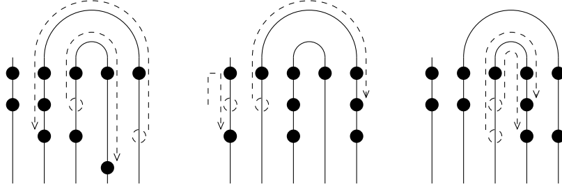
Figure 3.7: Moving beads on the linked abacus given in Figure 3.6.
