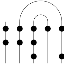
Figure 3.6: The partition (5, 4) on the linked abacus.
