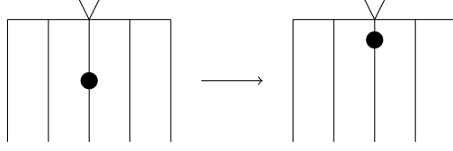
Figure 4.9: The movement of beads in Case 1.
