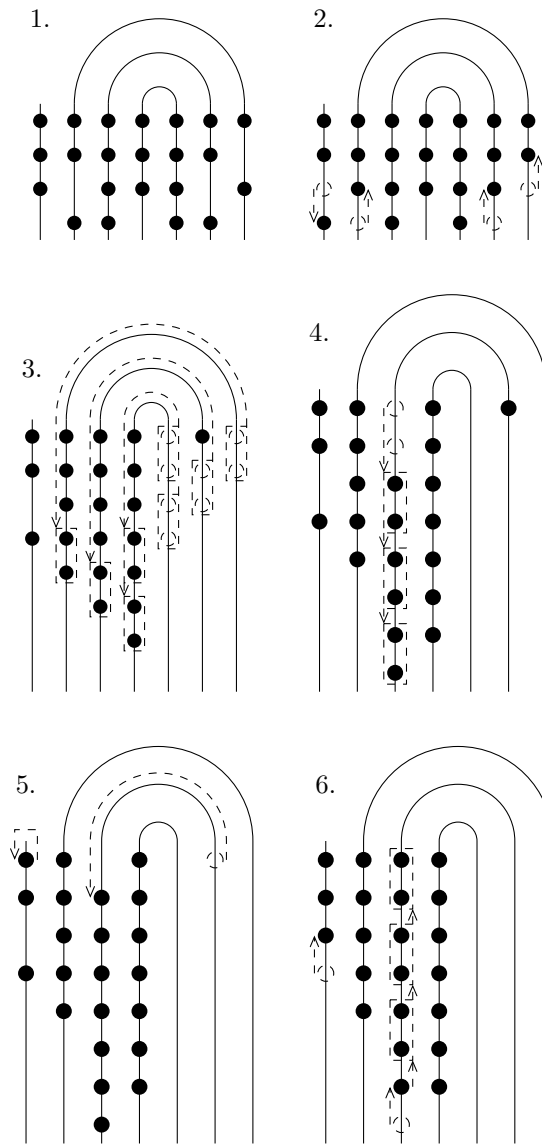
Figure 3.13: Constructing the b -reduction of (5^2, 4^2, 3, 2^3, 1) .
