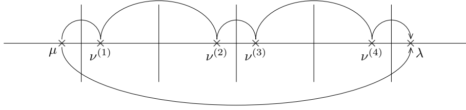
Figure 2.5: The construction of the \nu^{(i)} .
