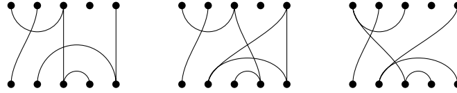
Figure 4.2: Three ways of representing the given set-partition.
