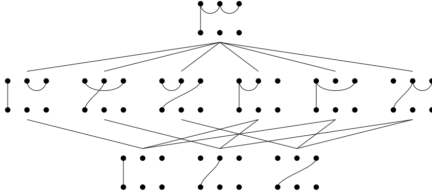
Figure 4.14: The Hasse diagram of I(3, 1) .
