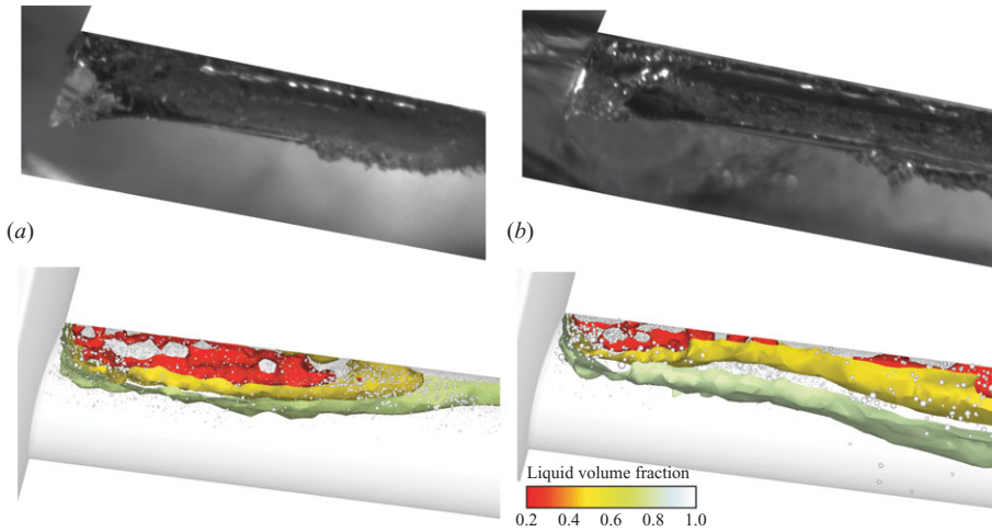
FIGURE 17. Side-view comparison between CCD images and model predictions for the vapour distribution on the surface of the large-scale nozzle: (a) incipient cavitation number case ( CN = 1.09 ) and (b) fully developed cavitation ( CN = 1.48 ) at nominal needle lift.
