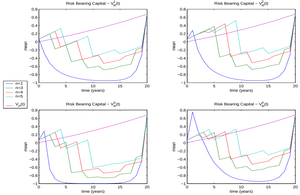
Figure 9: The mean of the risk bearing capital distribution resulting from the numerical experiment described in Figure 8. The risk bearing capital is calculated as (S_{tot} - V)/V , where V is the best estimate of the liability provided by the four dynamic reserving schemes described in section 4 and by the fair value V_P(t) .
