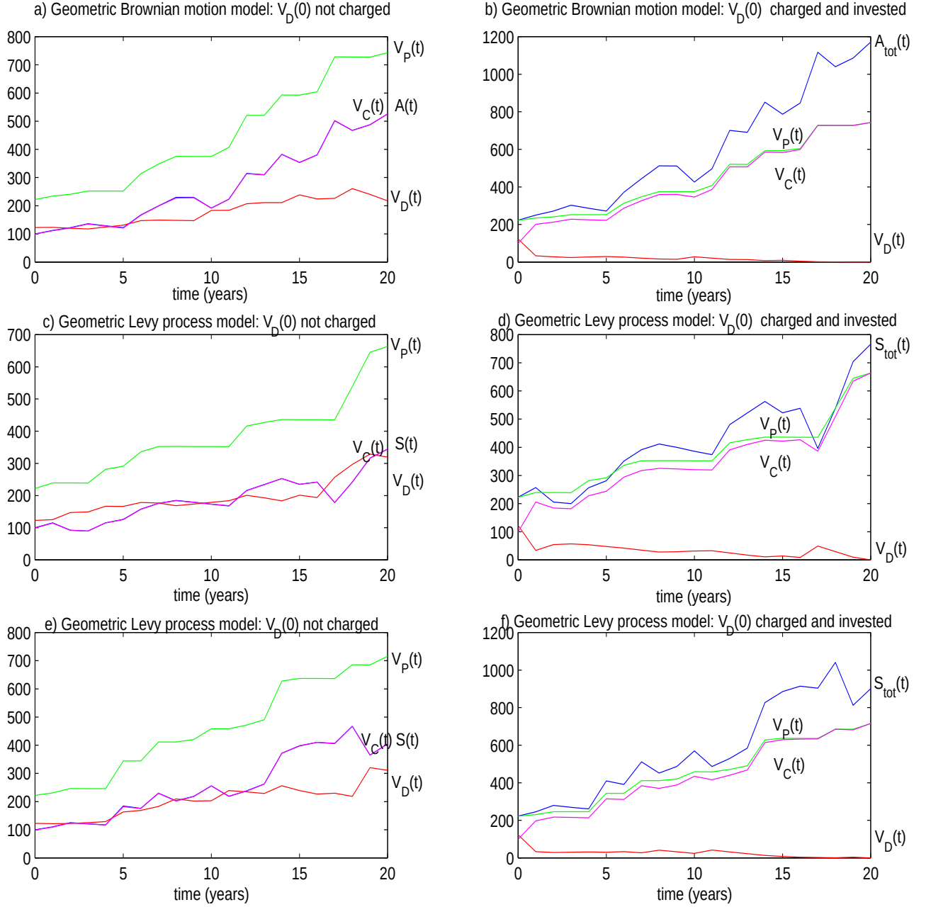
Figure 1: Scenario generation: a possible evolution of the reference fund and the fair value of the participating contract, the benefits and the default option. Panels (a)-(b) show one possible scenario under the geometric Brownian motion paradigm presented in section 2.1. Panels (c)-(d) and (e)-(f) illustrate two possible scenarios under the Lévy process paradigm discussed in section 3.1. The scenario generation has been obtained for the benchmark set of parameters under the real probability measure \mathbb{P} .
