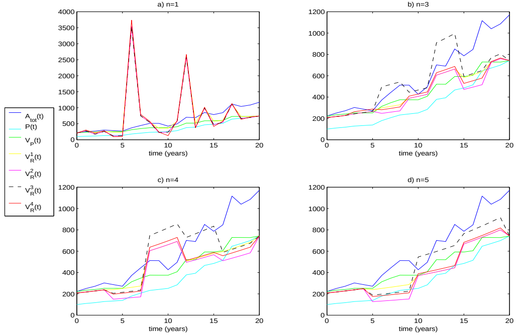
Figure 6: Scenario generation: the case of the dynamic reserves under the geometric Brownian motion paradigm. The trajectories of the market values are the same as in Figure 1.(b).
