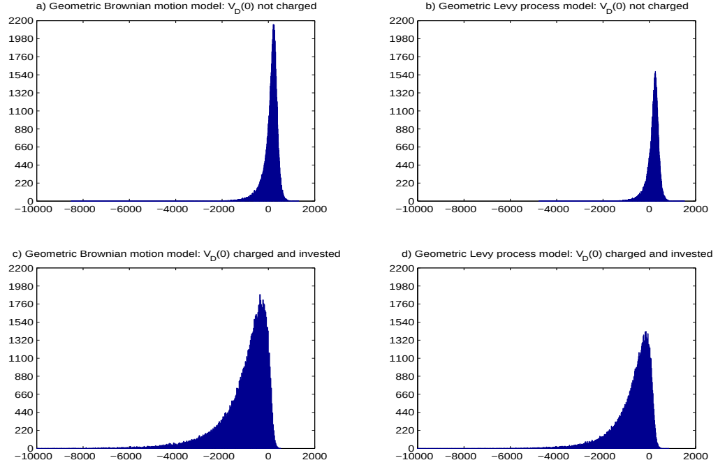
Figure 2: Shortfall distribution, \mathbb{P}(D(T) > 0) , for the benchmark set of parameters under the real probability measure, based on 100,000 scenarios.
