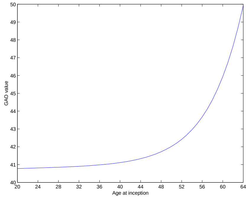
Figure 9: Time evolution of the guaranteed annuity option: the exponentially decaying volatility model.
