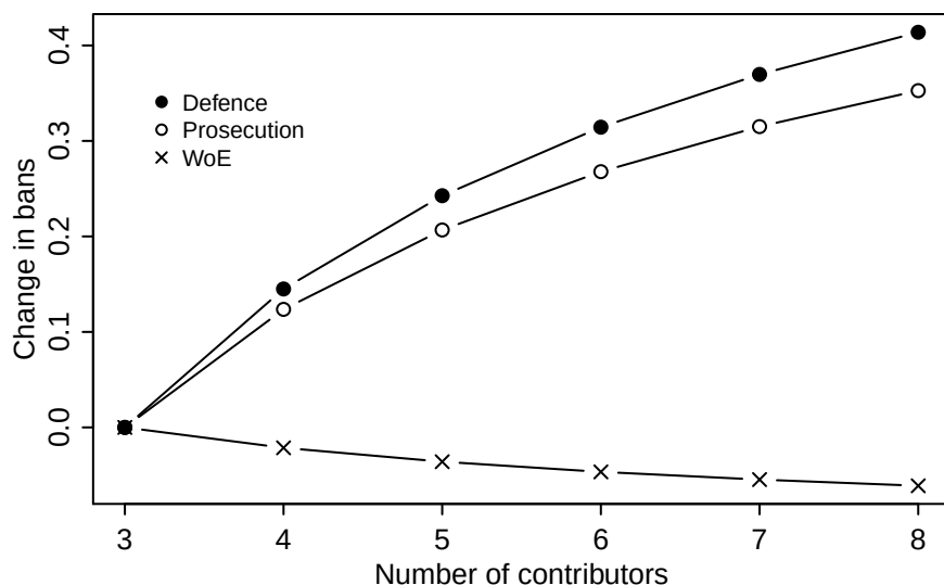
Fig. 8. The maximized log-likelihood functions based on combining MC15 and MC18 for varying number of contributors and hypotheses, relative to their value for three contributors and displayed in bans.
