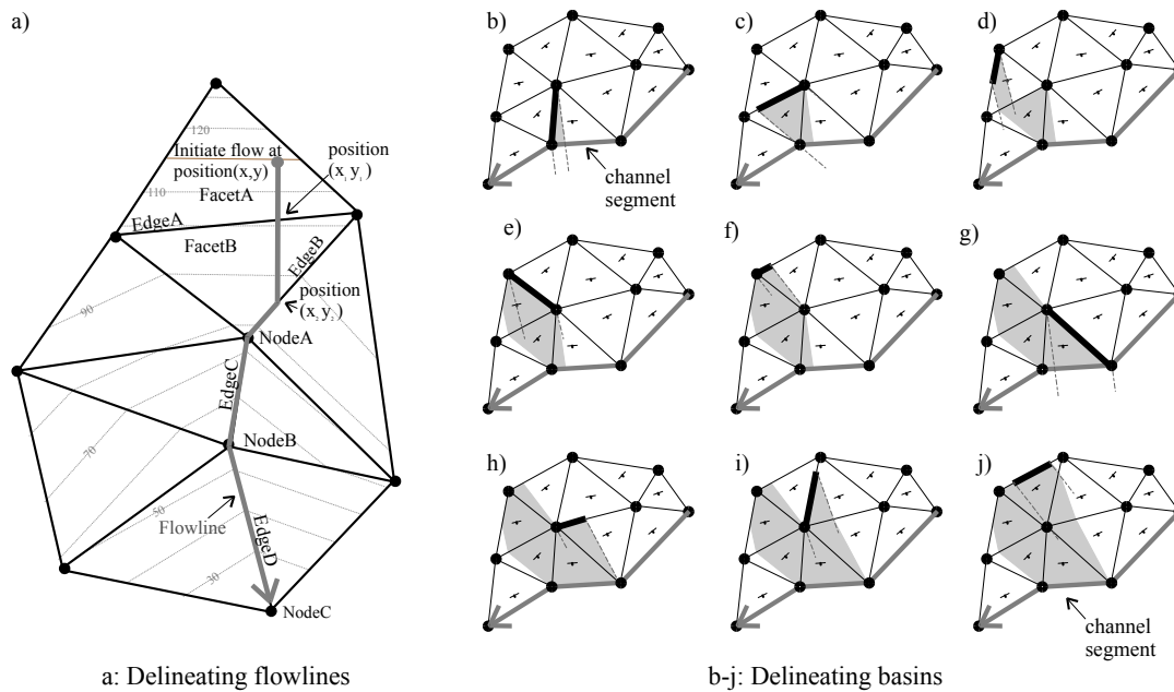
Figure 4: The piecemeal approach. (a) Delineating flowlines. Flow is initiated at the position x, y . FacetA can ascertain that the exit TIN element is EdgeA at position x_1, y_1 . EdgeA can ascertain that it is concave (thus a channel) and flow will leave through NodeA... and so on. In some cases, there may be more than one channel downslope from a node (stream divergence). (b-j) Delineating a basin. In this simplified example, the area that flows into the segment marked as “channel segment” is delineated (the area from one side only). This channel segment is the sole output of the facet above. This facet has two input edges that contribute to its sole output. In b the leftmost edge is taken (marked in black) and the area of the facet through which flow flows is marked (in grey), bounded by the line of steepest descent. In c, the facet above the previous edge has only one partial input edge (marked in black) from the facet above. The facet area to which this contributes is again marked. This process continues until the whole area that flows into the “channel segment” is delineated. For whole basins, this process starts from the lowest node of the basin, and works upwards to the watershed.
