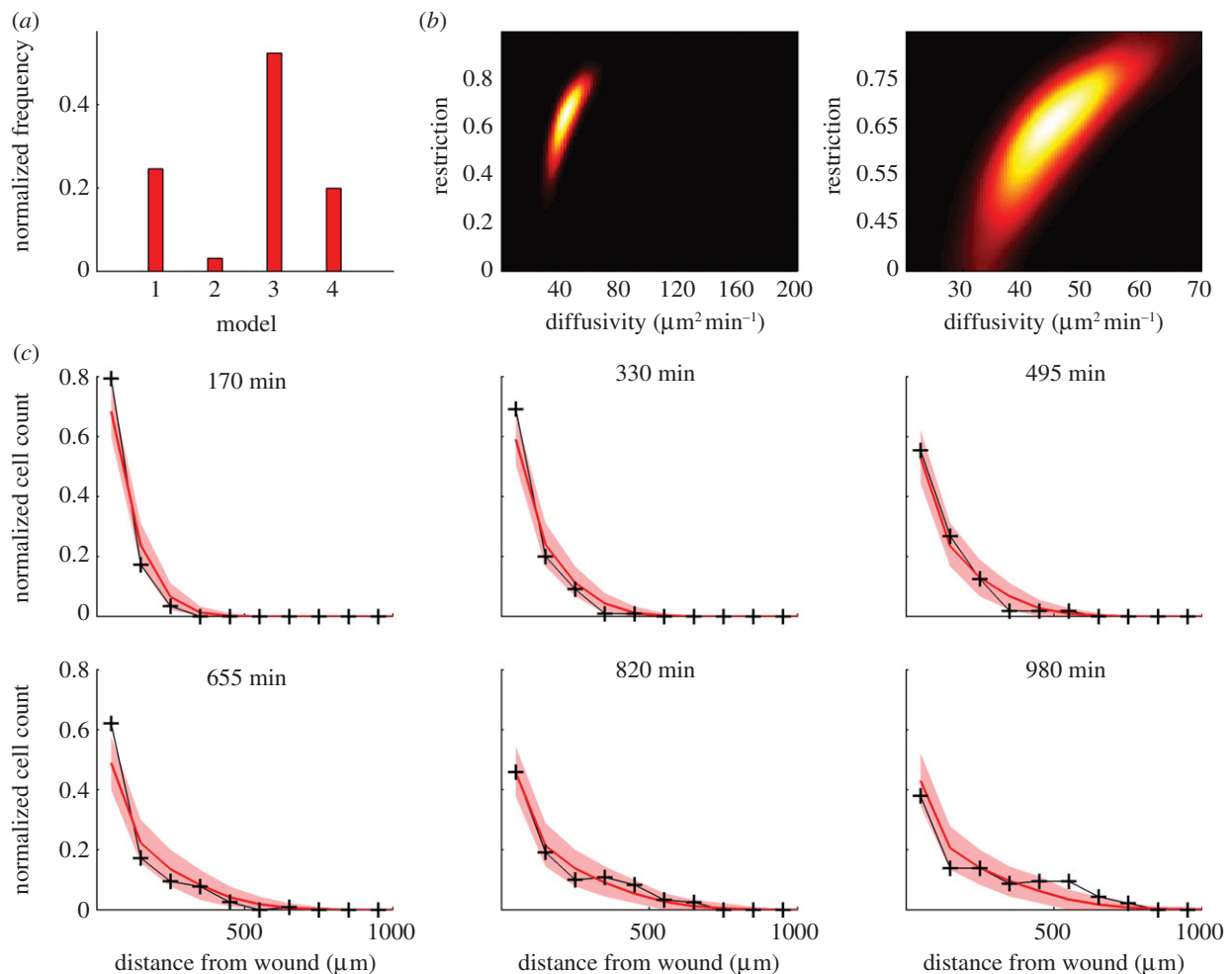
Figure 5. Identification of resolution phase neutrophil migration dynamics with restriction to preferred movement channels. (a) Model selection: model 1 is pure-diffusion; model 2 is drift–diffusion; model 3 pure-diffusion with restriction and model 4 is drift–diffusion with restriction. (b) Estimated joint distribution of parameters for model 3 (left panel over full support of the uniform prior and right panel zoomed in). (c) Simulation of the pure-diffusion with restriction model, model 3 (red), and comparison with experimental observations (black). The shaded region (red) shows the 90% confidence range obtained from 1000 simulations using the MAP estimates of the diffusion–restriction parameters.
