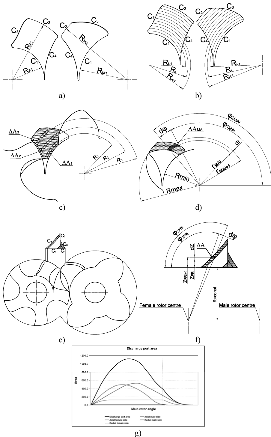
Figure 3 Principle of the discharge port area calculation
