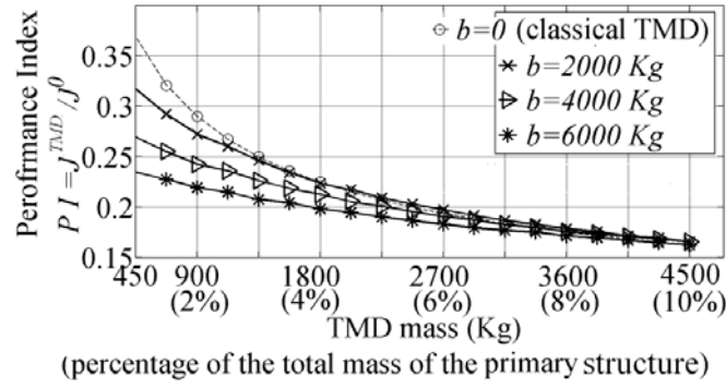
Figure 11. Achieved performance index versus the TMD mass for various values of the inerter constant b .
