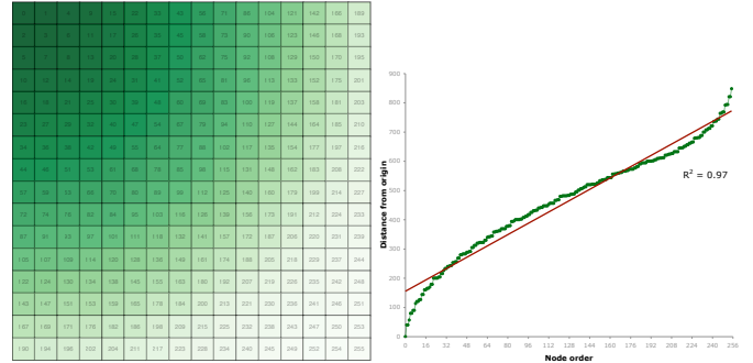
Fig. 4. OrderedSquarified layout of unit size nodes colored by order. Euclidean distance from the top-left corner (origin) is approximately linearly proportional to node order. Variations from linearity are due to forcing a circular distribution into an enclosing rectangle.
