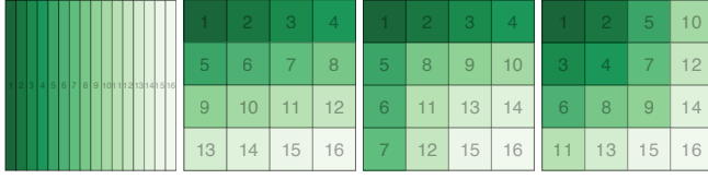
Fig. 2. Slice and dice [21], strip [2], squarified [5] and ordered squarified layouts of 16 ordered nodes of unit size. The readability scores of the four layouts are 1.0, 0.625, 0.375 and 0.125 respectively (1 indicates no angular change, 0 indicates every jump between sequential nodes requires an abrupt angular change).
