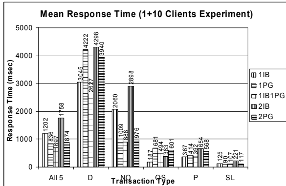
Figure 6. The mean transaction times for single DBMS configurations (1IB, 1PG), diverse DBMSs pair (1IB1PG) and homogenous DBMS pairs (2IB, 2PG) for each transaction type and for all transactions
