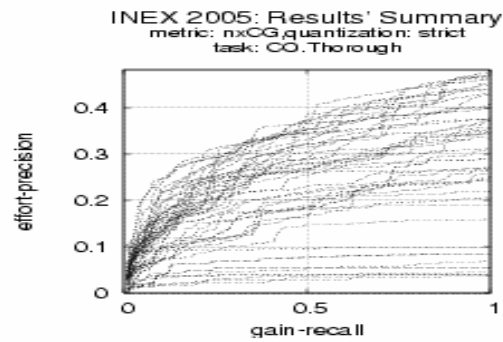
Fig. 2 Metric nxCG(50), Quantization: strict, Overlap=off
