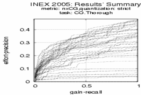
Fig. 1 Metric nxCG(25), Quantization: strict, Overlap=off
