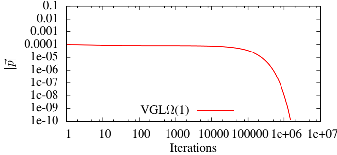
Fig. 2. Convergence for VGLΩ(1) using the same parameters that caused VGL(1) to diverge, and \alpha = 10^{-3} . This algorithm demonstrates that it is possible to have proven convergence for a critic learning algorithm with a greedy policy and general function approximation.
