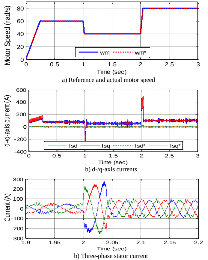
Fig. 9. Performance of nested-loop neural network controller in power converter switching environment
