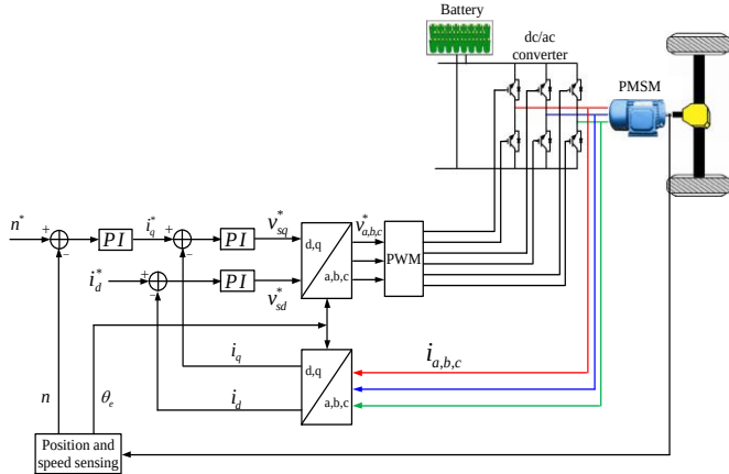
Fig. 1. Configuration and control of a PMSM in EDV application
