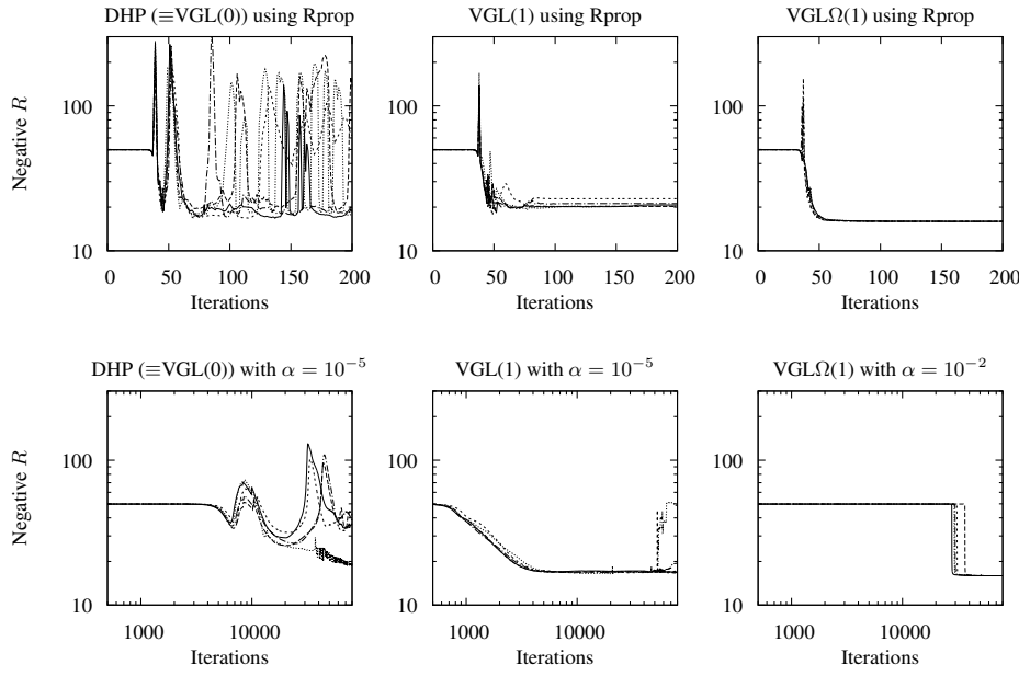
Figure 7.2 Results show learning progress for 5 typical random weight initialisations, for the problem of trying to learn 10 different trajectories. Results show increasing effectiveness (particularly in reduced volatility) for the three learning algorithms being considered, in the order that the graphs appear from left to right. The top row of graphs are all using RPROP to accelerate learning. The bottom row of graphs all use a fixed step-size parameter \alpha .
