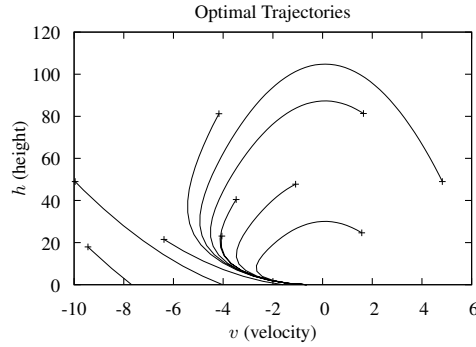
Figure 7.1 State space view of a sample of optimal trajectories in the Vertical Lander problem. Each trajectory starts at the cross symbol, and ends at h = 0 . The u -dimension (fuel) of state space is not shown.
