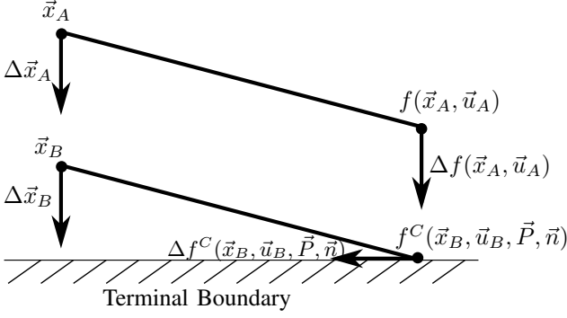
Fig. 5: This diagram shows how the derivatives of the model function f(\vec{x}, \vec{u}) radically change as the agent approaches a terminal boundary. The straight line segment from \vec{x}_A to f(\vec{x}_A, \vec{u}_A) represents a state transition that is not intersecting the terminal boundary. If the start of this line segment is perturbed in the direction of the arrow \Delta \vec{x}_A then its other end will move in the direction indicated by the arrow \Delta f(\vec{x}_A, \vec{u}_A) . The line segment below, however, which starts at \vec{x}_B , does reach the terminal boundary. If the start of this line segment is moved in the direction of \Delta \vec{x}_B , then its end will move in a perpendicular direction, as indicated by the arrow \Delta f^C(\vec{x}_B, \vec{u}_B, \vec{P}, \vec{n}) . This indicates that (\partial f^C / \partial \vec{x})_A is very different from (\partial f / \partial \vec{x})_B , and hence this needs treating carefully in the ADP algorithms.
