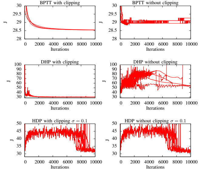
Fig. 6: Vertical-Lander solutions by BPTT, DHP and HDP using \Delta\tau = 1 . Each graph shows five curves, i.e. five experimental trials.
