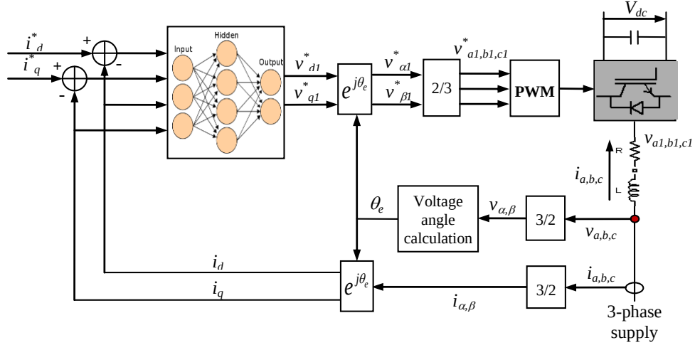
Figure 2: GCC neural vector-control structure.
