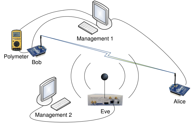
Figure 3: Test-bed topology
