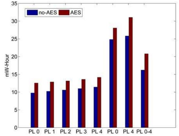
Figure 10: Energy consumption in milliWatt-Hour for different power levels (PL) of the three scenarios
