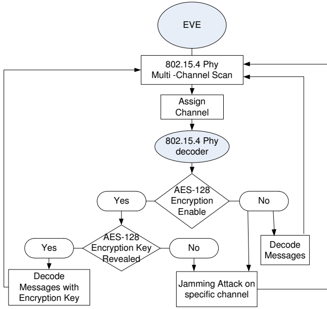
Figure 6: The attacker flowchart model
