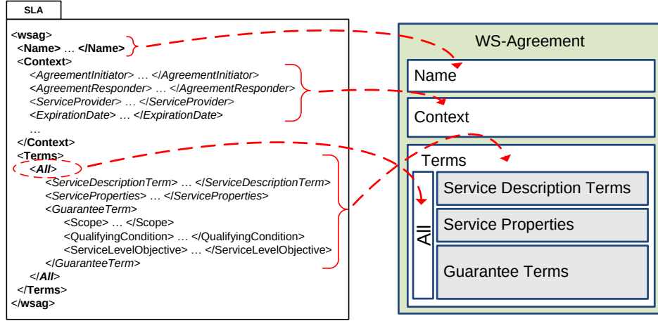
Figure 2: WS-Agreement structure
