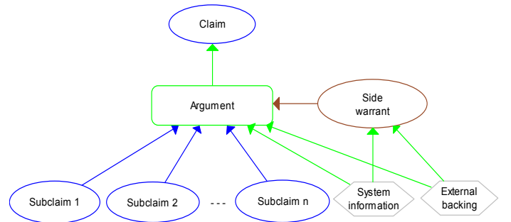
Figure 3. General CAE Block Structure.
