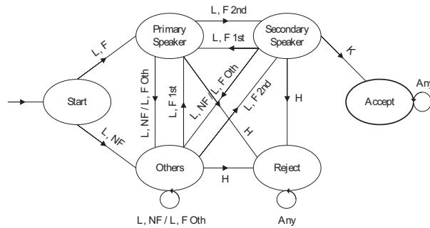
Fig. 2.7. FSM for conversational scene. L – low activity intensity; H – high activity intensity; F – facial shot; NF – non-facial shot; 1st, 2nd, Oth – speaker clusters; K – acceptance condition satisfied; Any – any shot (adapted from [53]).
