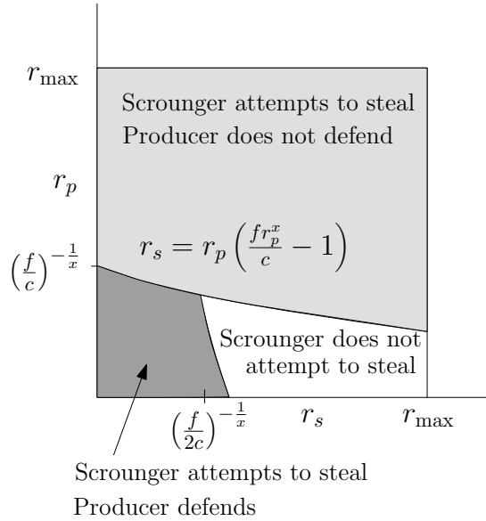
Figure 5: Behavioural outcomes of the game for v(r) = fr^x, x < -1 .
