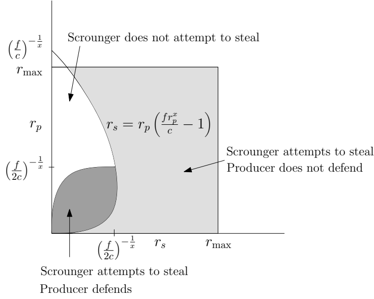
Figure 4: Behavioural outcomes of the game for v(r) = fr^x, x \in (-1, 0) .
