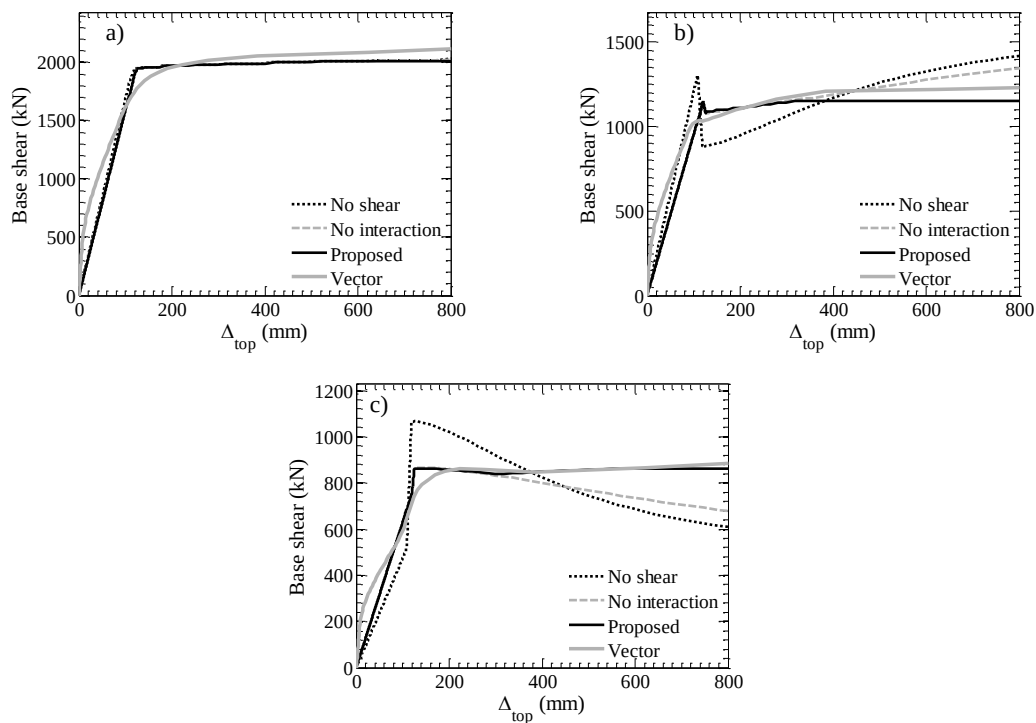
Figure 12. Base shear vs. top displacement responses of the cantilever wall structure for (a) the entire structure, (b) the long wall and (c) the short wall
