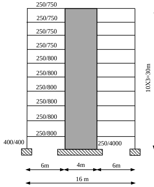
Figure 13. Geometry of the wall-frame structure
