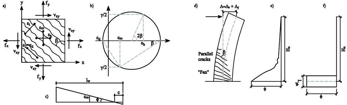
Figure 2. (a) Truss analogy model for RC elements with parallel compression struts; (b) Mohr's circle, representing the strain state at the center line of the wall; (c) strain profile showing \varepsilon_m and \phi . Plastic hinge method: (d) crack pattern; (e) true curvature profile; (f) plastic curvature profile assumed in plastic hinge method (Beyer et al. 2011)
