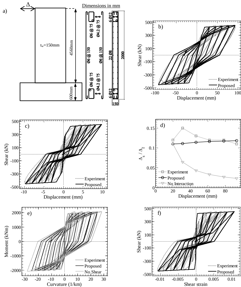
Figure 8. RC structural wall WSH3 by Dazio et al. (2009): (a) structural configuration; (b) shear force vs. total displacement; (c) shear force vs. shear displacement; (d) variation of shear-to-flexural displacement ratio with imposed top displacement demand; (e) base moment vs. curvature; (f) shear force vs. distortion in the plastic hinge region
