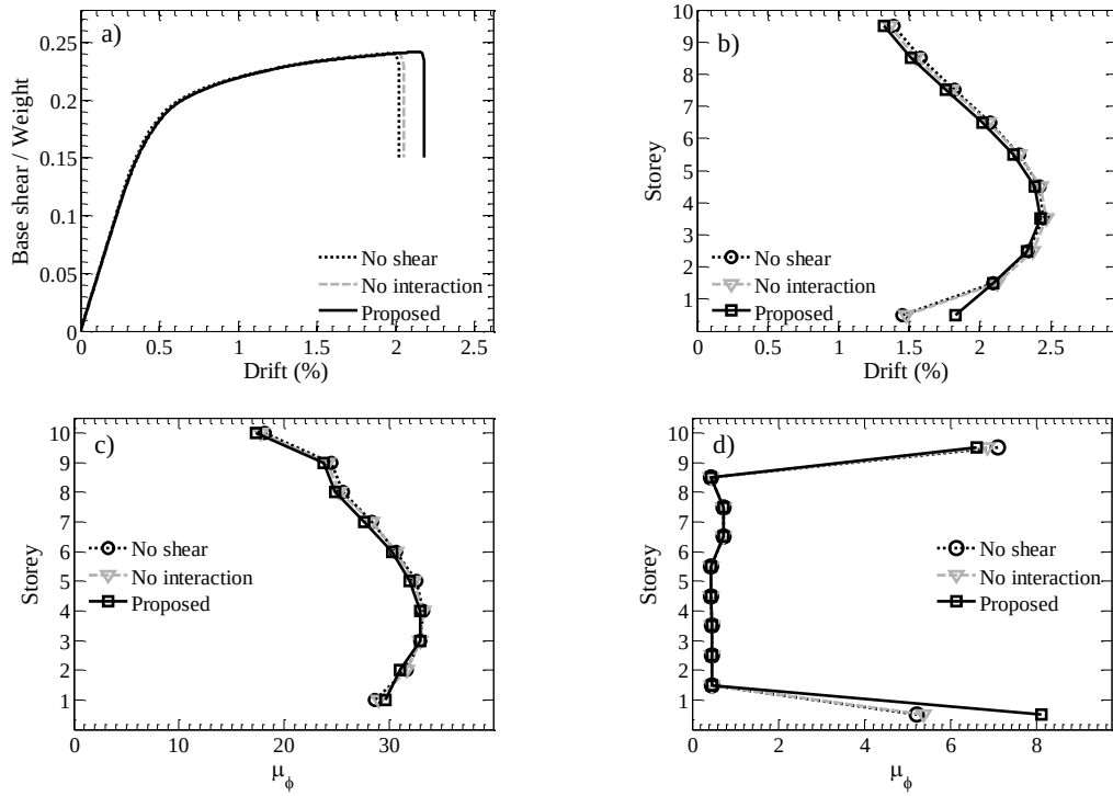
Figure 14. Pushover analysis results: (a) base shear over weight vs. top displacement over total height; (b) maximum normalized interstorey drifts at 2% normalized top displacement demand; (c) maximum beam curvature ductility demands and; (d) maximum column curvature ductility demands at a top displacement corresponding to an average drift of 2%
