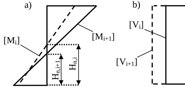
Figure 9: Case study of a wall member with varying height of contra-flexure: (a) bending moment diagram; (b) shear force diagram in two subsequent analysis steps
