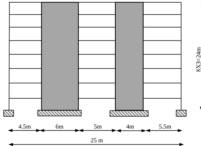
Figure 11. Geometry of the cantilever wall with two slender RC walls of different lengths
