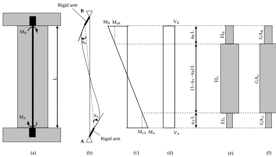
Figure 3. Beam-column element with shear-flexure interaction: (a) RC wall; (b) finite element; (c) moment diagram; (d) shear diagram; (e) flexural sub-element; (f) shear sub-element
