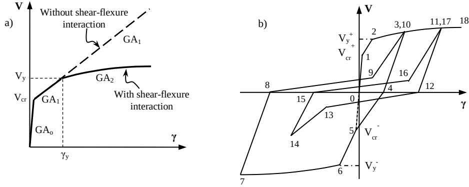
Figure 5. Shear force-shear strain ( V - \gamma ) hysteretic response: (a) initial and modified envelope curve; (b) hysteretic model
