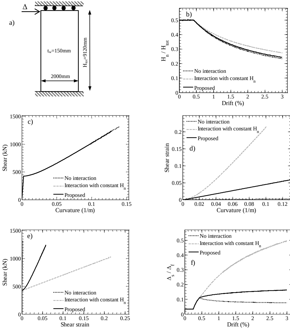
Figure 10. RC structural wall in double bending: (a) structural configuration; (b) variation of cantilever height with lateral drift; (c) shear force vs. base curvature; (d) base shear strain vs. base curvature; (e) shear force vs. base shear strain; (f) variation of shear-to-flexural top displacement ratio with lateral drift
