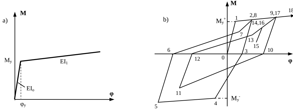
Figure 4. Moment-curvature ( M-\phi ) hysteretic response: (a) bilinear envelope curve; (b) hysteretic model
