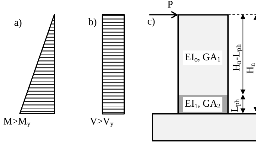
Figure 7: Cantilever wall: a) moment diagram; b) shear force diagram; c) flexural and shear stiffness distribution after shear cracking and flexural yielding under monotonic loading
