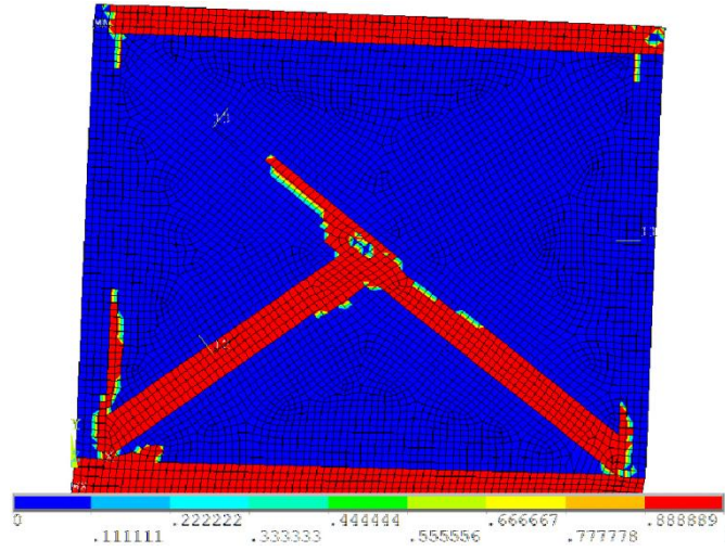
Figure 13 TF wall with full connections of masonry infills: stress ratios ( \sigma/f_m ).
