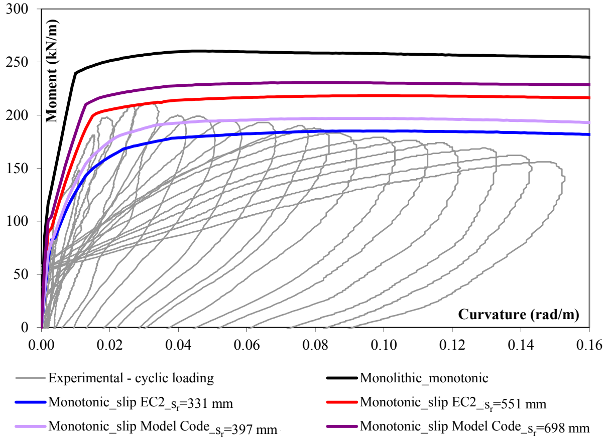
Figure 11: Comparison of the moment – curvature response curves derived for the various crack spacing estimations with the experimental moment – curvature hysteresis loops.
