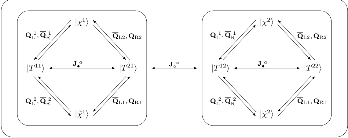
Figure 2. The eight massless excitations form two \mathfrak{psu}(1|1)_{\text{c.e.}}^4 multiplets. The four bosons T^{\dot{a}a} are charged both under \mathfrak{su}(2)_\bullet and \mathfrak{su}(2)_\circ , while the four fermions \chi^a, \tilde{\chi}^a are in the fundamental representation of \mathfrak{su}(2)_\circ only. Again we indicate the charges whose action corresponds to the outermost arrows of the diagram, while the innermost ones follow by Hermitian conjugation. Note how \mathfrak{su}(2)_\circ relates the two \mathfrak{psu}(1|1)_{\text{c.e.}}^4 modules, yielding a single irreducible representation of \mathcal{A} , denoted by a box.
