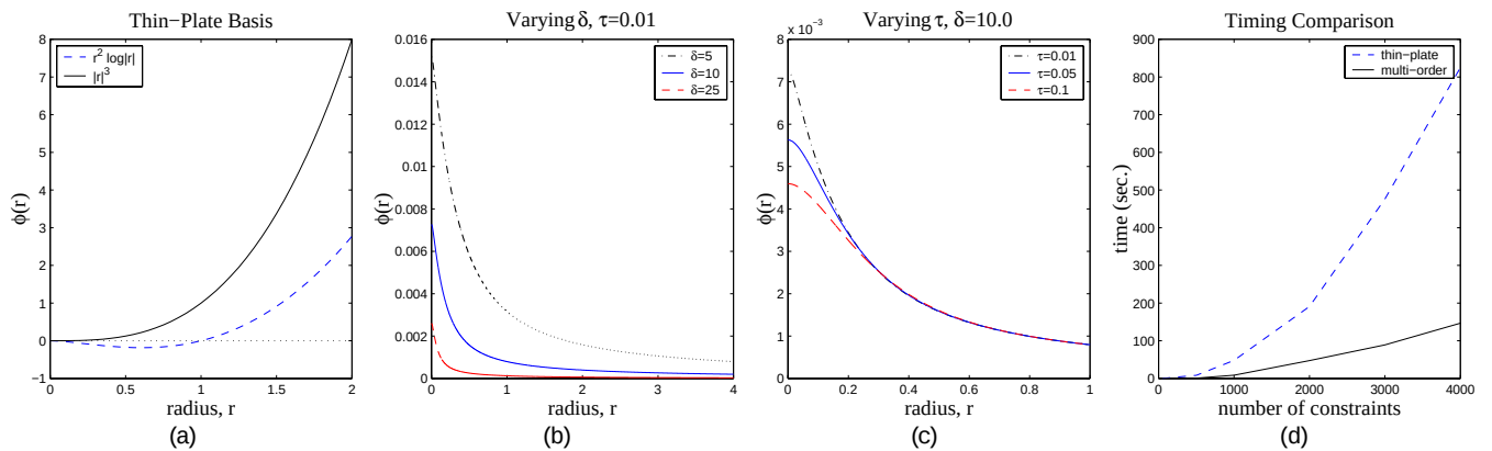
Fig. 4. (a) Cross sections of radially symmetric basis functions for |r|^2 \log|r| and |r|^3 . (b) and (c) Cross sections of basis functions for a combination of first, second, and third order smoothness for various values of \delta and \tau . (d) Comparison of running times to solve for weights for the thin-plate and for the multi-order basis functions.
