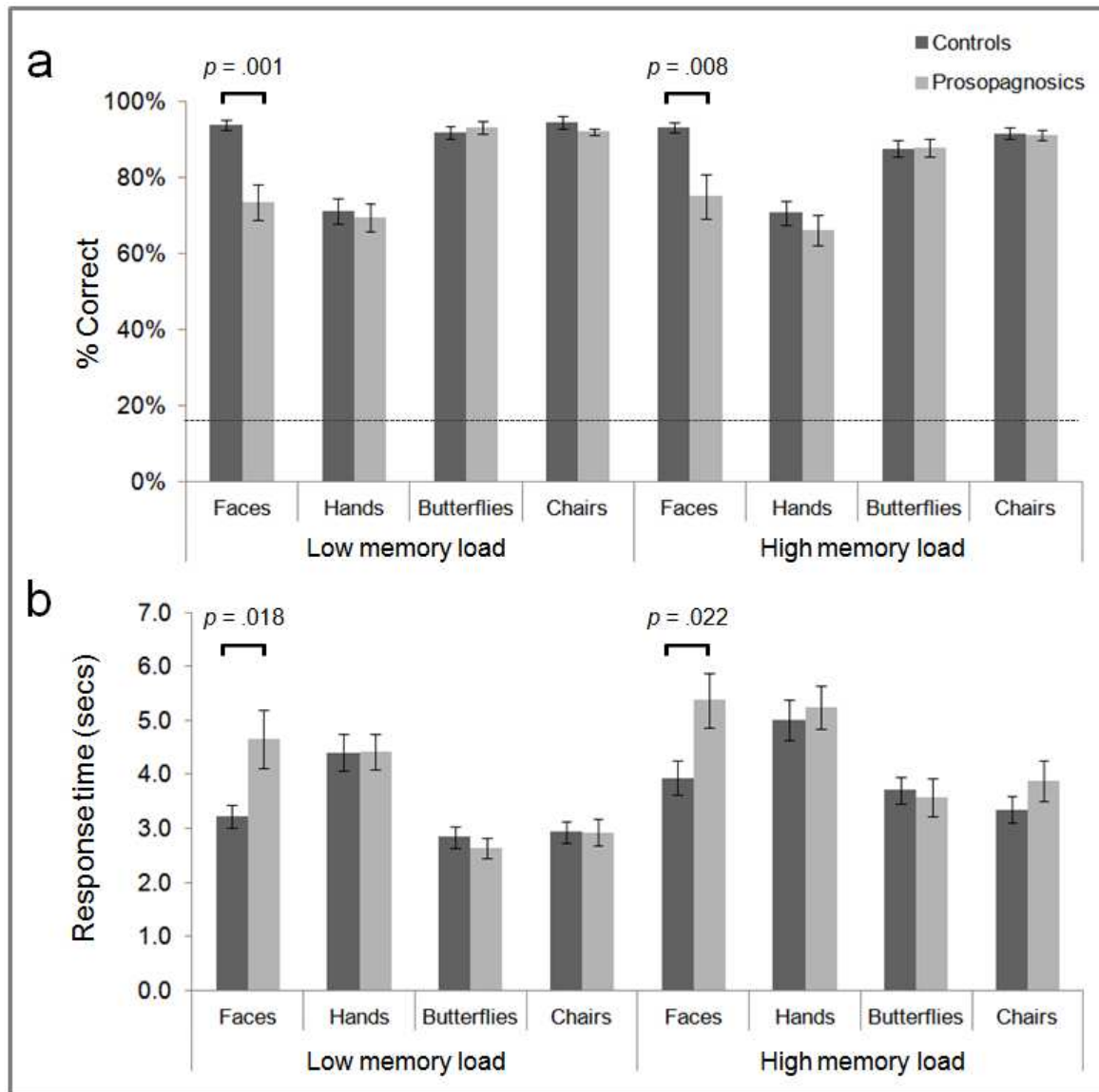
Figure 3: (a) Accuracy data for the prosopagnosic and control groups. The dashed line indicates chance performance (16.7%) in the 6-alternative-forced-choice match-to-sample procedure. (b) The mean response times for the prosopagnosic and control groups. Both the accuracy and response time analyses indicate that prosopagnosics were selectively impaired at faces, and that this deficit is comparable following short and long retention-intervals.
