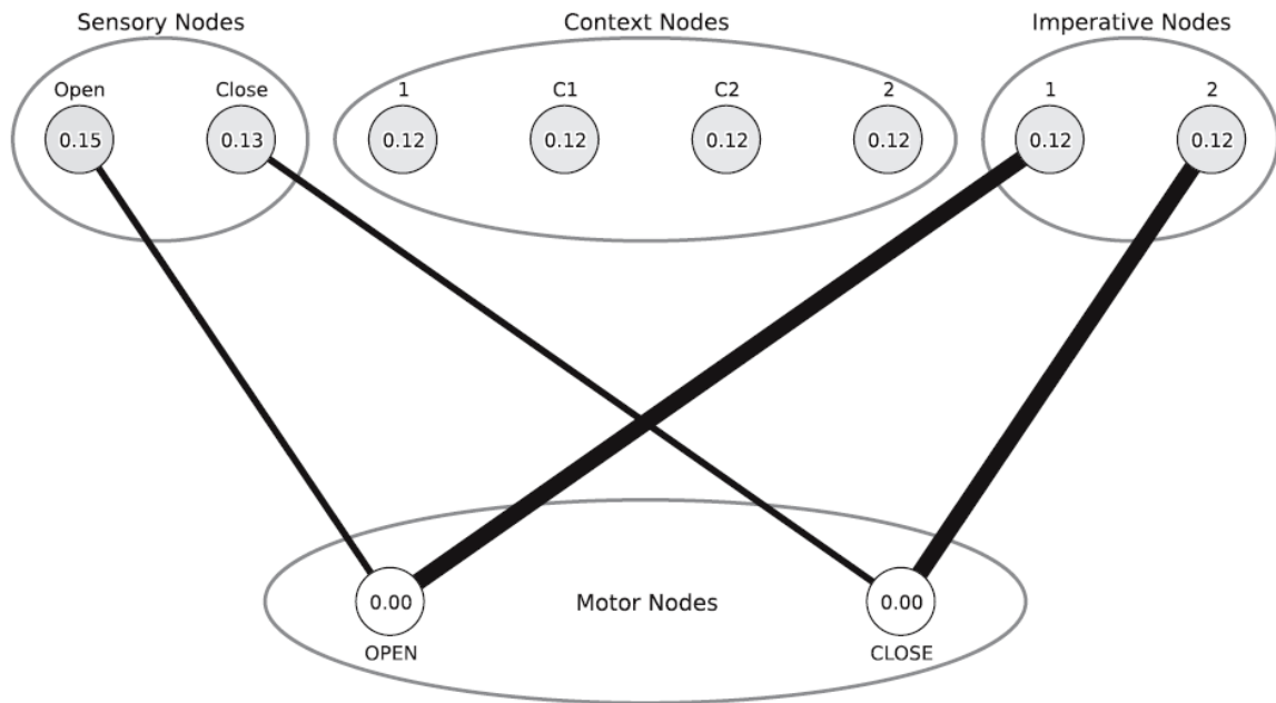
Figure 2: Architecture of the model, showing associations between nodes prior to learning.
