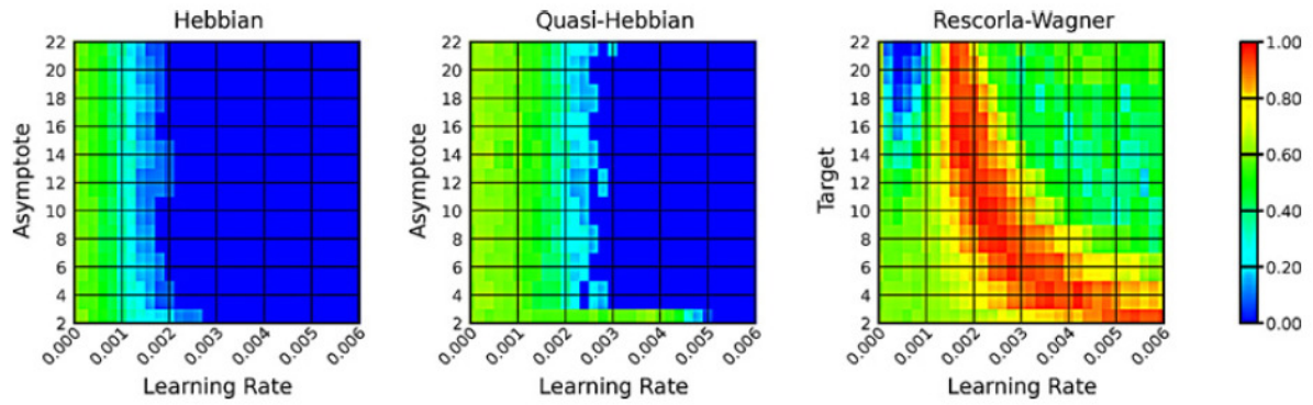
Figure 5: Fit of the model with different learning rules to the qualitative effects in the subject data of Cook et al. [7, Experiment 2]. These plots effectively show the ability of the model to simultaneously fit all three effects considered in Figure 4. Red regions correspond to parameter settings where the model replicates all effects found in the subject data. They correspond to the overlap between red regions in Figure 4 left, red regions in Figure 4 centre, and green regions in Figure 4 right, for each learning rule.
