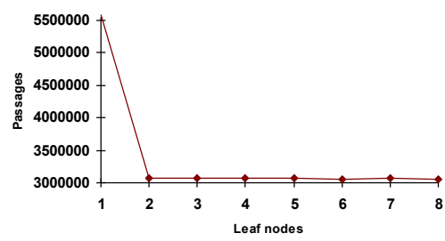
Fig 21. BASE1 [ whole topic ]: Retrieval efficiency, passages processed for 1000 documents overall
