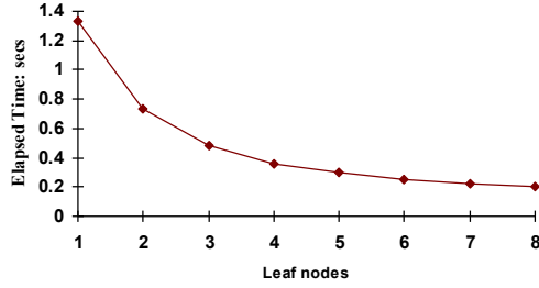
Fig 3. BASE1 [ title only ]: Retrieval efficiency, average elapsed time in seconds for 1000 documents per node
