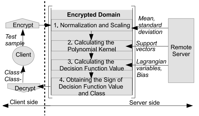
Fig. 3. The block diagram of proposed PP SVM.
