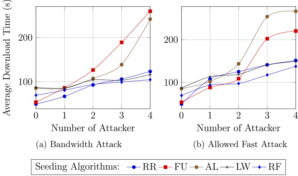
Figure 4: File transfer of a 100 MiB file with a piece size of 64 KiB via BitTorrent with a seeder that has 5 Mbps upload limit. Subfigure (a) shows a normal bandwidth attack and subfigure (b) shows a bandwidth attack combined with the allowed fast attack.
