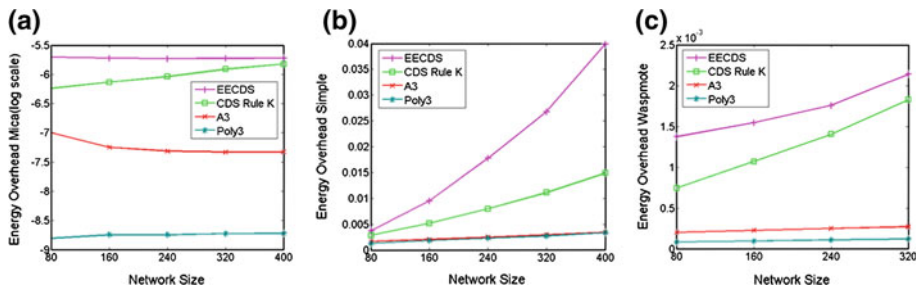
Fig. 7 Impact of varying node densities on energy overhead for a Mica, b Simple and c Wasp mote
