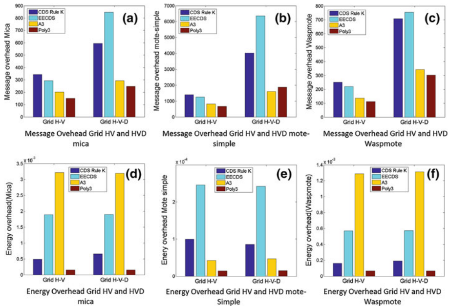
Fig. 5 Performance comparison under Grid HV and Grid HVD topologies. a Message overhead grid HV and HVD mica. b Message overhead grid HV and HVD mote-simple. c Message overhead grid HV and HVD Wasp mote. d Energy overhead grid HV and HVD Mica. e Energy overhead grid HV and HVD mote-simple. f Energy overhead grid HV and HVD Wasp mote
