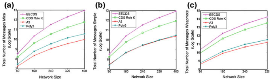
Fig. 6 Impact of varying node densities on message overhead for a Mica, b Simple and c Wasp mote
