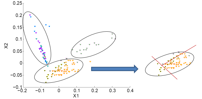
Fig. 1. An example of Activity Recognition by Clustering based Classification (AR-CbC). The axes X_1 and X_2 show the first two principal components of features. Similar activity instances are grouped into one cluster. A learning method is applied for classification within each cluster that separates the overlapping activities.
